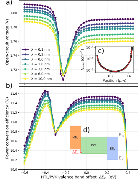
Fig. 1. (a) Open-circuit voltage and (b) Power conversion efficiency as a function of the HTL/PVK interface valence band offset, for different values of the effective length \lambda of the defects spatial distribution, with constant total areal trap density of 10^{11} \text{ cm}^{-2} . (c) Example of fitting of experimental spatial distribution of traps from [4] using (1). (d) Schematic of the solar cell band alignment.
