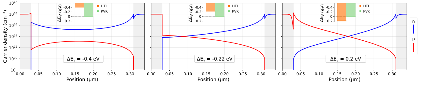
Fig. 2. Electron (blue) and hole (red) densities for different HTL/PVK interface band offsets, considering the PVK/ETL interface perfectly aligned ( \Delta E_C = 0 ). All figures are obtained at 1.71 V, i.e. at the open circuit voltage of the case with \Delta E_V = -0.22 eV, and \lambda = 1 nm.
