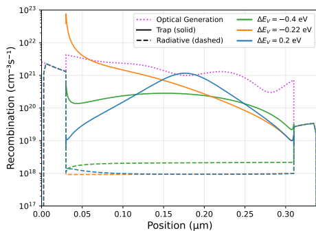
Fig. 3. Optical generation and recombination profiles for the three alignment cases described in figure 2.
