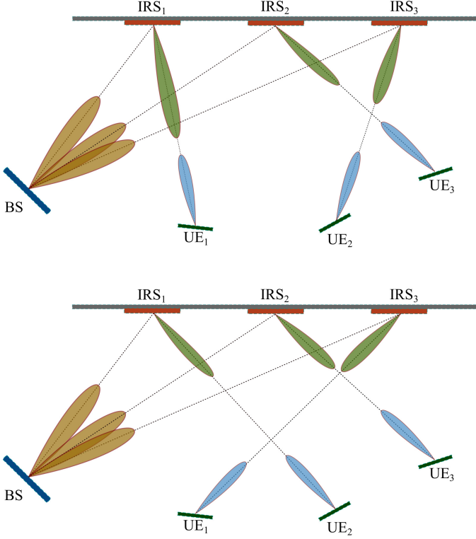
Figure 2: Two possible configurations for a network with N = K = 3 . The top configuration corresponds to the map \nu_a(1) = 1 , \nu_a(2) = 3 , and \nu_a(3) = 2 , while the bottom configuration corresponds to the map \nu_b(1) = 3 , \nu_b(2) = 1 , and \nu_b(3) = 2 .
