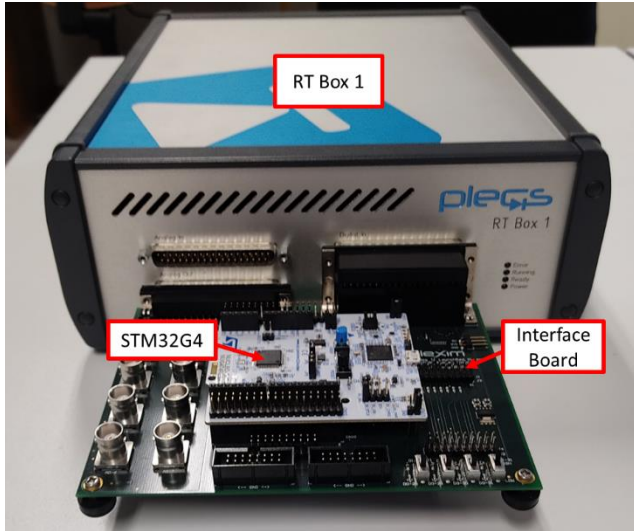
Fig. 17 HIL test rig consisting of the PLECS RT Box 1 and the NUCLEO-STM32G474RE.
