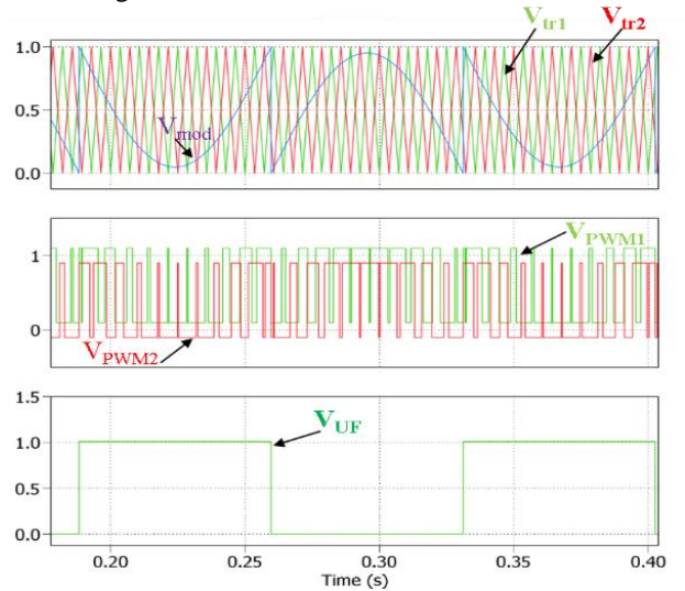
Fig. 6 Modulation strategy for two interleaved switching legs and the unfold leg (PLECS® simulation).
