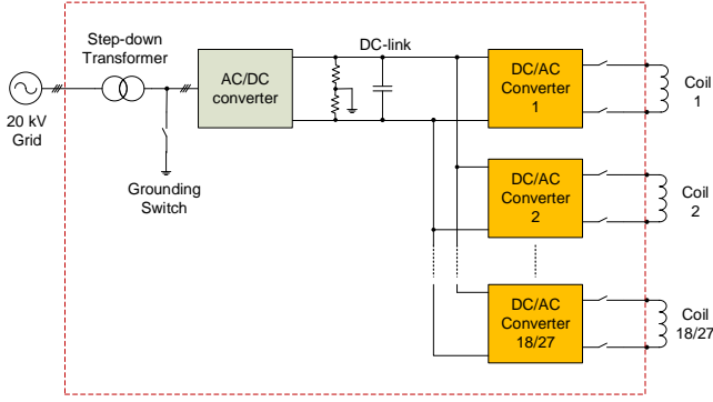
Fig. 2 Block schematic of the multi-converter power supply for the DTT NAS coils.
