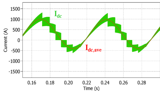
Fig. 13 dc link current I_{dc} and its average I_{dc,\text{ave}} over a switching period.
