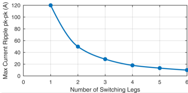
Fig. 15 Variation of maximum current ripple in the NAS coil considering different numbers of switching legs.
