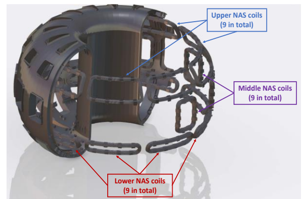
Fig. 1 Arrangement of the DTT NAS coils inside the vacuum vessel. The final configuration includes 3 \times 9 = 27 NAS coils in total.
