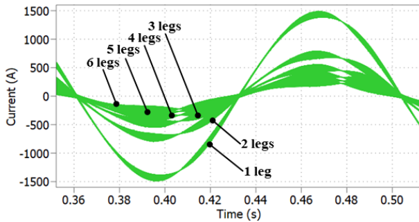
Fig. 14 Variation in the leg current of a single switching leg considering different numbers of switching legs.
