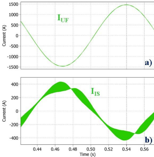
Fig. 11 Single phase inverter current. a) output current of the unfold switching leg ( I_{UF} ). b) output current of a single switching leg of the interleaved switching pole ( I_{IS} ).
