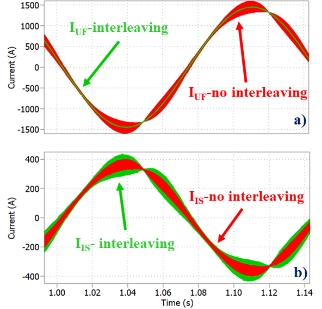
Fig. 16 Impact of the phase interleaving on the NAS coil current and phase switching leg current. a) current in the NAS coil with and without phase interleaving. b) current in one of the switching legs with and without phase interleaving.
