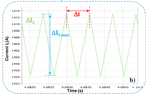
Fig. 12 a) Load current I_L simulation result. b) zoomed view of the ripple current behavior.
