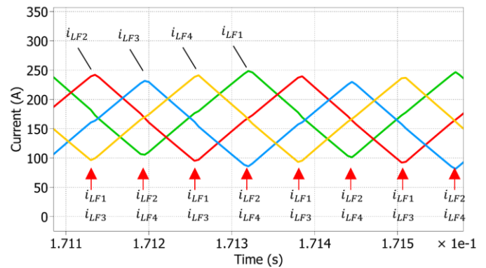
Fig. 22 Detail of Fig. 21 showing the current ripple and the optimal sampling time.
