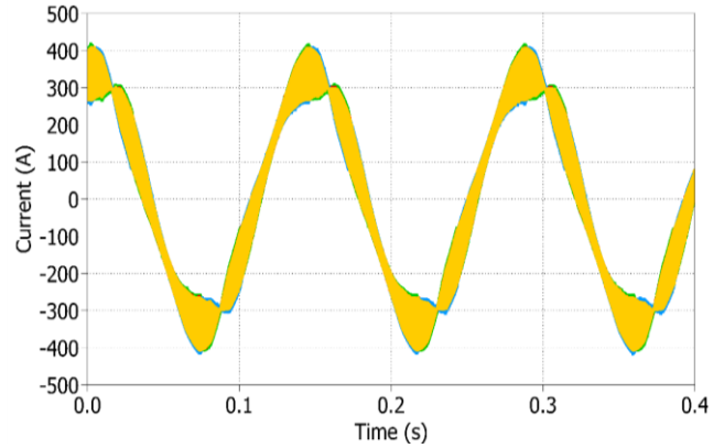
Fig. 21 Currents in the four switching legs (traces are overlapped) during the HIL implementation.
