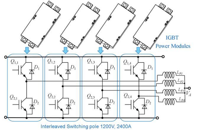
Fig. 7 Interleaved switching pole with 4 switching legs for the arrangement of the single-phase inverter.
