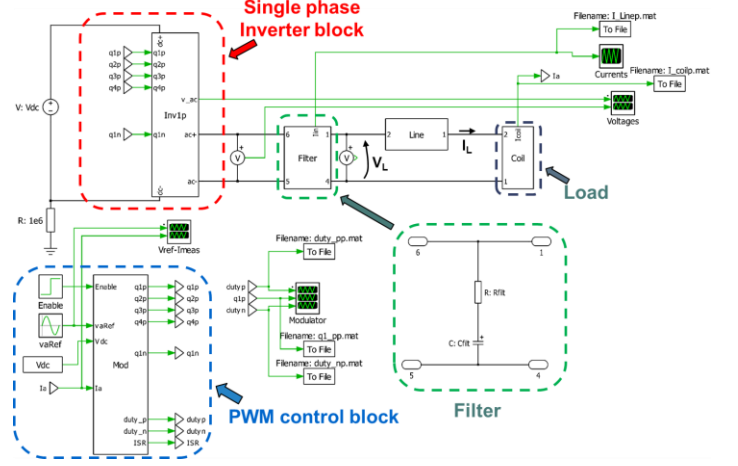
Fig. 8 Block schematic of the global supply system for the single NAS coil used in PLECS® simulation runs.
