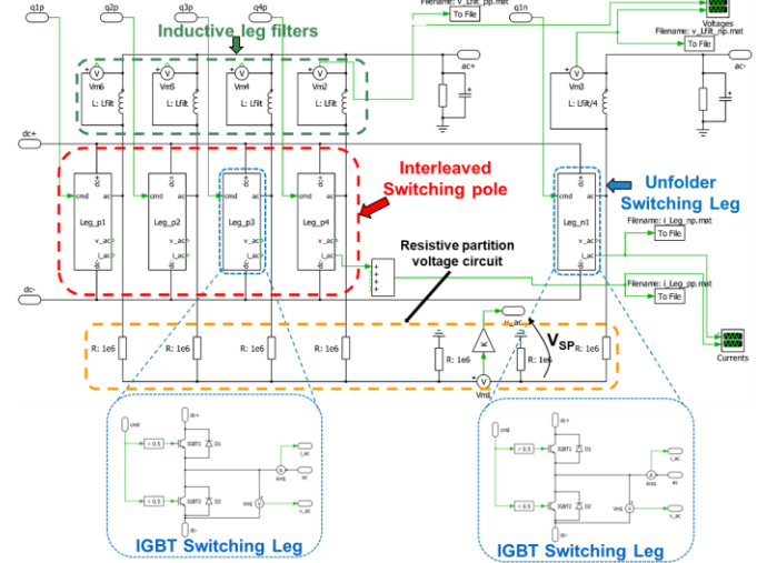
Fig. 9 Block schematic of the single-phase inverter topology with an interleaved switching pole and unfolder switching leg used in PLECS® simulation runs.
