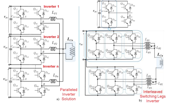
Fig. 4 (a) Parallel inverter topology (b) Interleaved switching leg inverter circuit.
