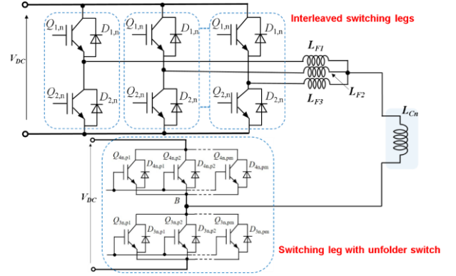
Fig. 5 Single-phase inverter topology with interleaved switching pole and unfold switching leg.
