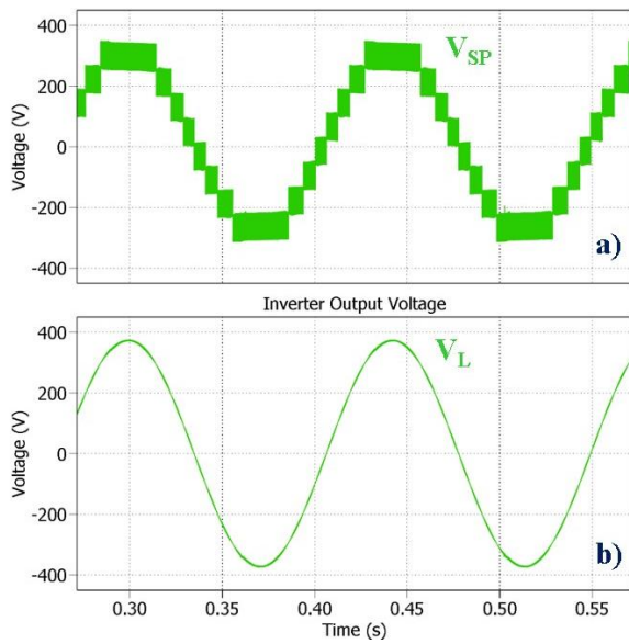
Fig. 10 Output voltage of the single-phase inverter without filter (a) and with the RC filter (b).
