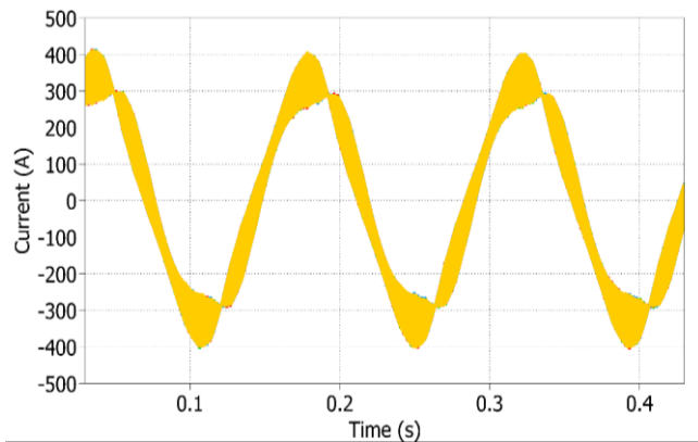
Fig. 20 Current in the four switching legs during the digital PLECS implementation.
