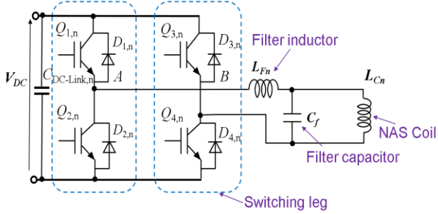
Fig. 3 Standard inverter topology with IGBTs for the DTT NAS coil power supply.
