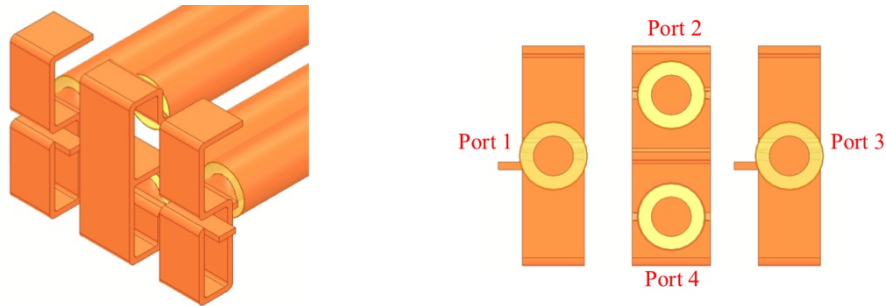
Figure 12.a – The three double strap array Figure 12.b – Port assignment
