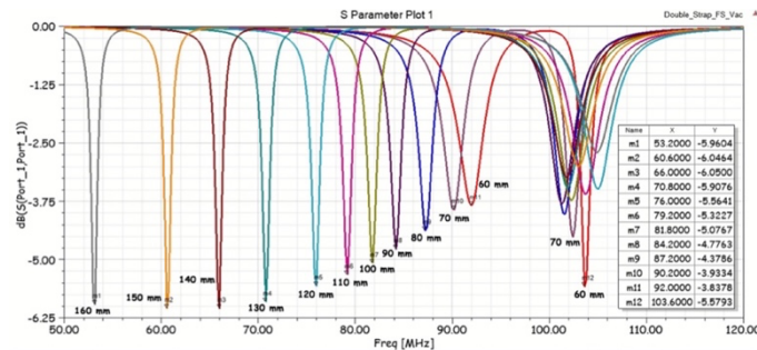
Figure 9 – Resonant Launcher, Reflection Coefficients
