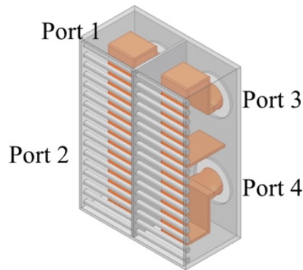
Figure 7 – Four parallel straps with Faraday screen
