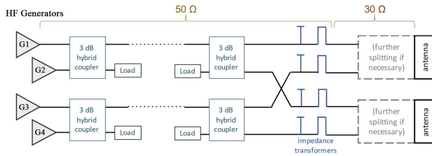
Figure 1 – ICRF System for DTT Schematic
