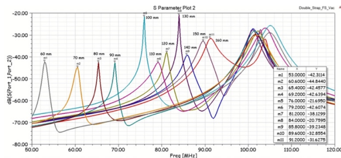
Figure 10 – Resonant Launcher, Cross-coupling Coefficients
