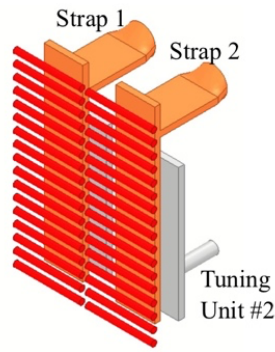
Figure 8 –Resonant double strap launcher
