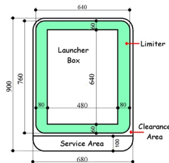
Figure 2 – DTT port cross-section sizes
