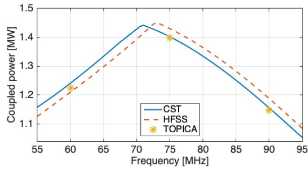
Figure 3 – Benchmark of HFSS and CST simulations with homogeneous dielectric against TOPICA results for a three-strap antenna in front of a DTT reference plasma.
