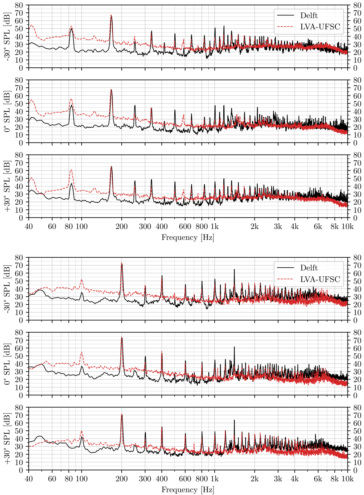
Fig. 9 5000 RPM and 6000 RPM spectra for -30^\circ , 0^\circ and 30^\circ polar angles.
