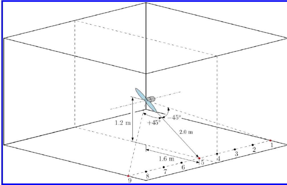
Fig. 2 UFSC microphone array.
