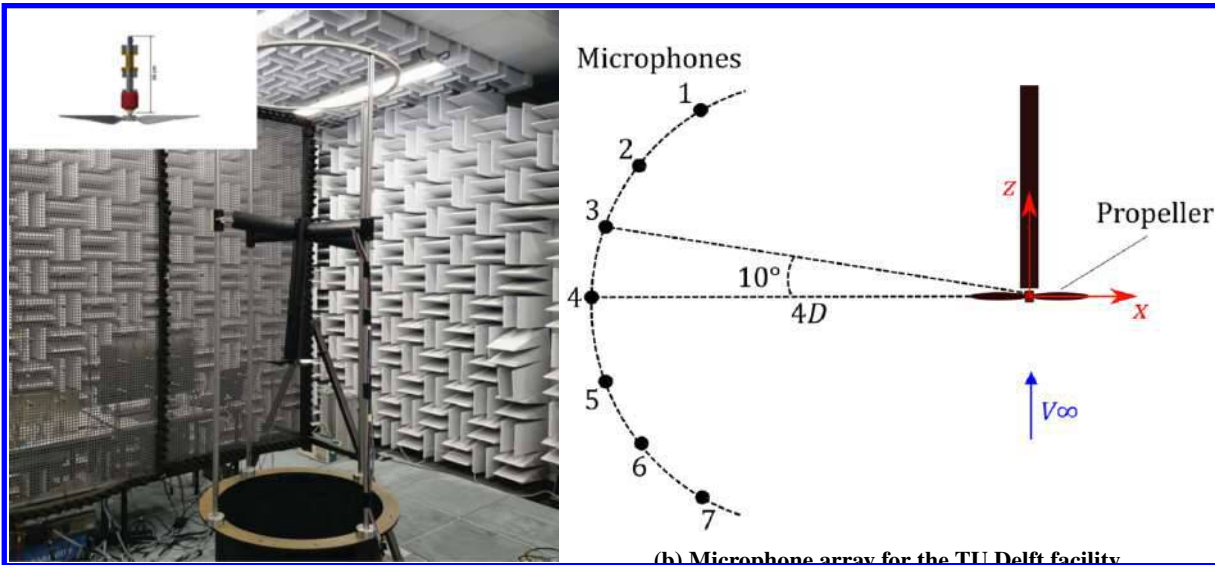
(a) Picture of the TU Delft facility.
