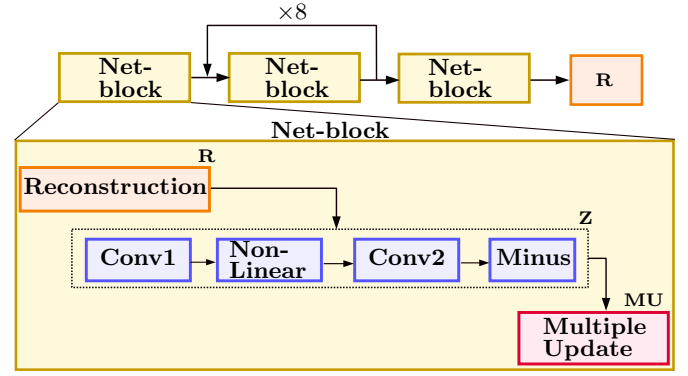
Fig. 2. ADMM-CSNet architecture. Multiple Net-blocks perform a full reconstruction step. The second block processes data iteratively 8 times, emulating the ADMM algorithm. Inside a Net-block, data passes through a first reconstruction layer R , then into two convolutional layers which perform the ADMM auxiliary variable update ( Z blocks), followed by a multiple update module MU .
