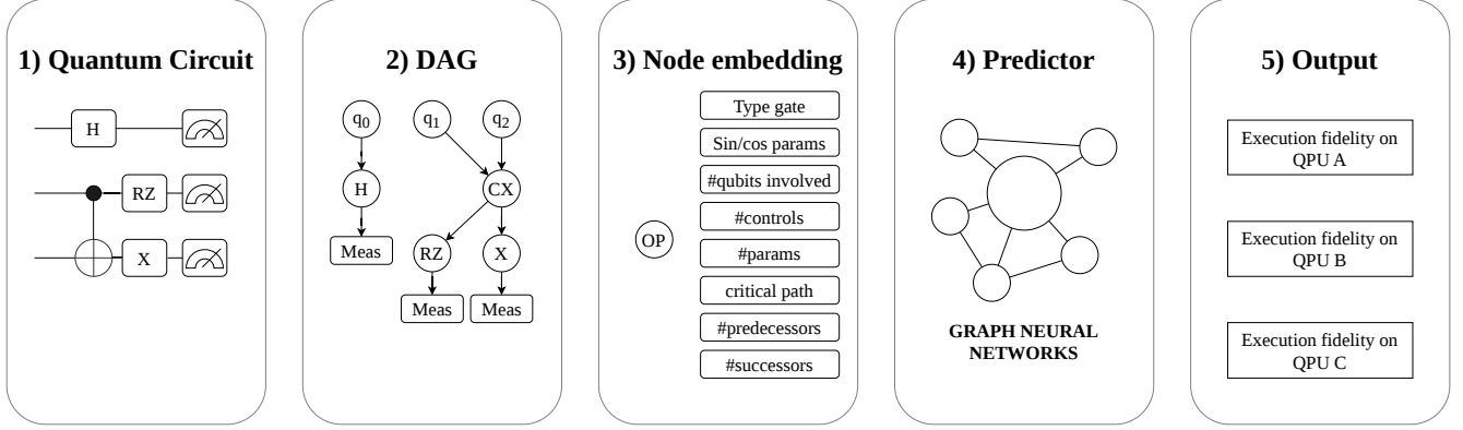
Fig. 3: Fidelity-based quantum device selection using a GNN. Starting from an input quantum circuit, the framework constructs a DAG, converts gate information into a numerical node representation, and feeds the resulting feature vector to a GNN. The model then estimates the execution fidelity for all considered target devices in parallel.
