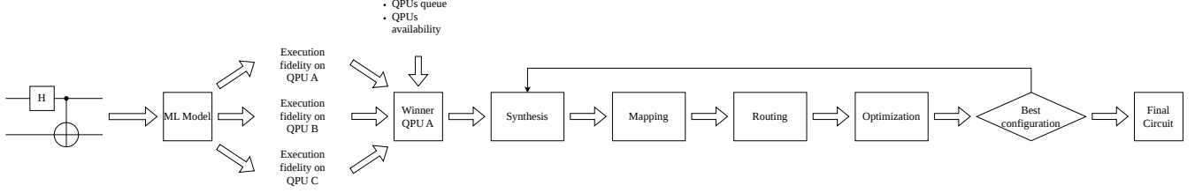
Fig. 2: Workflow for selecting the most suitable quantum device for a given program and compiling it accordingly. The device is chosen based on the fidelity predictions of a ML model, avoiding individual compilation for all candidate devices.
