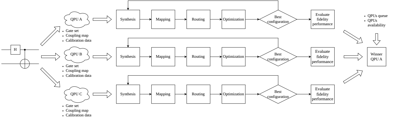
Fig. 1: Workflow for selecting the most suitable quantum device for a given program. The program is compiled for each available QPU, and the chosen fidelity/performance metric is evaluated using device-specific calibration data. The final device is then selected by maximizing the considered performance metric while accounting for additional factors such as queue length and availability.
