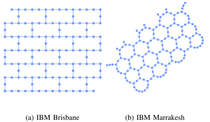
Fig. 4: Coupling maps of considered superconducting devices.
