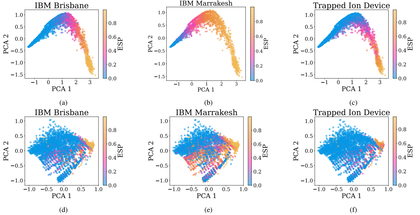
Fig. 6: PCA results for the three considered devices. The top row, panels (a)–(c), shows the latent representations produced by the convolutional component of the GNN model projected onto the first two principal components. The bottom row, panels (d)–(f), shows the feature representations used by the MQT Predictor projected onto the first two principal components.
