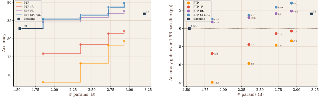
(a) DecisionxR1 accuracy under unstructured pruning. All pruned models start from 3B, while 1.5B is shown as the smaller dense baseline.
