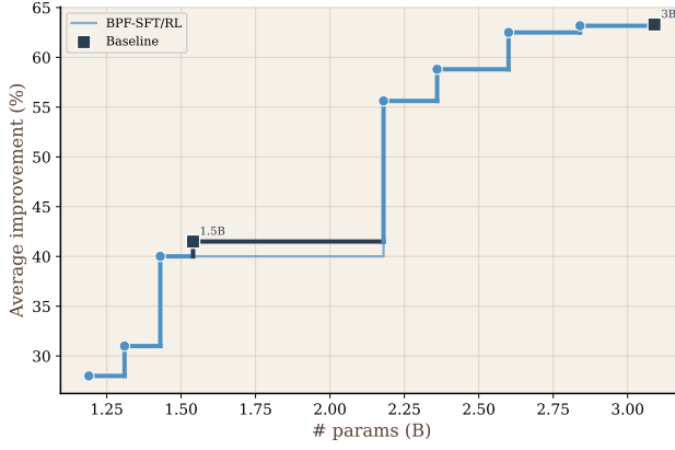
Figure 6: DecisionxR1 pruning with fixed MPCxR1, using both 3B and 1.5B as starting checkpoints for BPF-SFT/RL.
