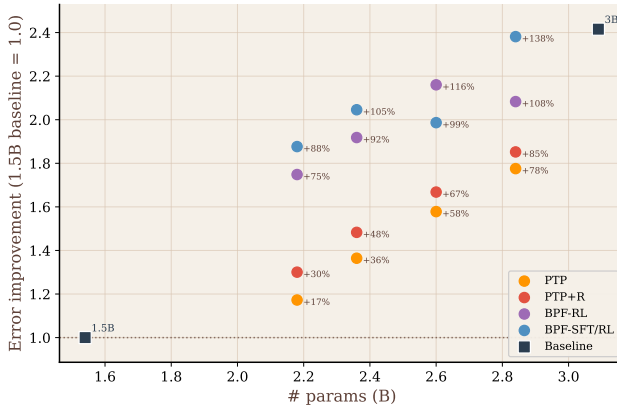
Figure 7: Average task-error improvement of pruned DecisionxR1 models initialized from 3B, measured relative to the 1.5B baseline. The score averages the relative improvement across the four task errors ( E_c , E_v , E_r , E_s ).
