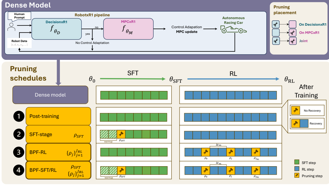
Figure 1: Overview of the pruning strategies and placement in our pipeline.
