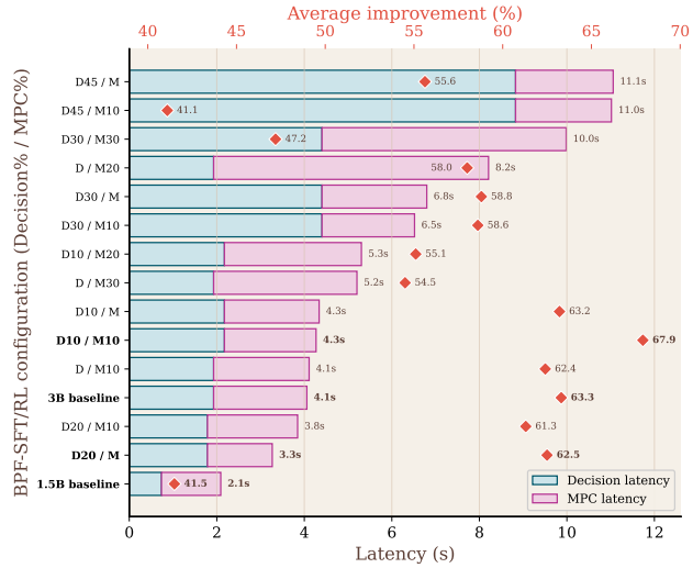
Figure 5: End-to-end latency of the full pipeline. The bottom x-axis reports measured latency, while the top x-axis reports corresponding task-performance from Fig. 3. Pareto configurations are highlighted in bold .
