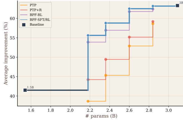
Figure 2: Average control-adaptability improvement over the default MPC controller as in [7] versus model size.
