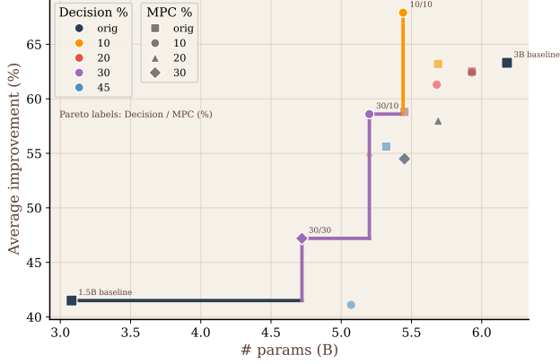
Figure 3: End-to-end control-adaptability trade-off when pruning both DecisionxR1 (colors) and MPCxR1 (shapes).
