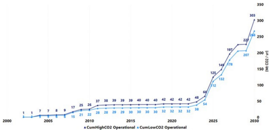
Fig. 10 Cumulated captured MtCO 2 /year for operational CC projects (high vs low capacity scenarios). Source: Our elaborations on IEA's 2023 CCUS Projects Database
