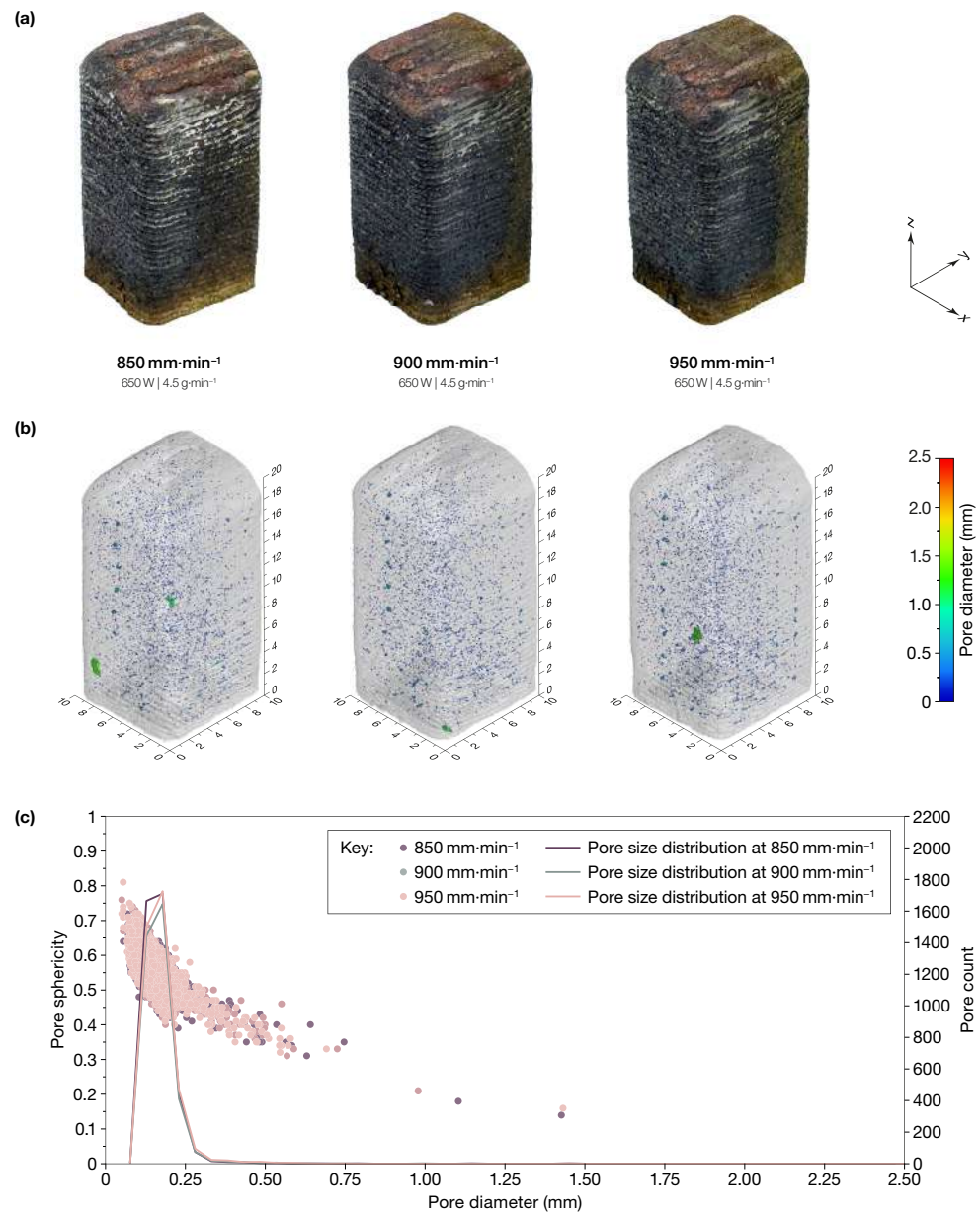
Figure 6. (a) Surface aspect, (b) pore distribution and (c) pore diameter vs. sphericity of samples produced with different travel speed values. The laser power was P = 650 W and the powder mass flow rate was Q_p = 4.5 g·min -1 .
