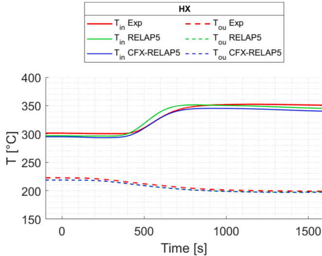
Fig. 16. Experimental vs RELAP5 vs coupling HX temperature comparison (ADP06).
