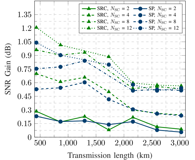
Fig. 8. SNR gain obtained by evolving from subcarrier-independent to joint pilot-based CPE approaches. Results are displayed as a function of the transmission distance. R_P \approx 2\% and a total launch power of 0 dBm were used.
