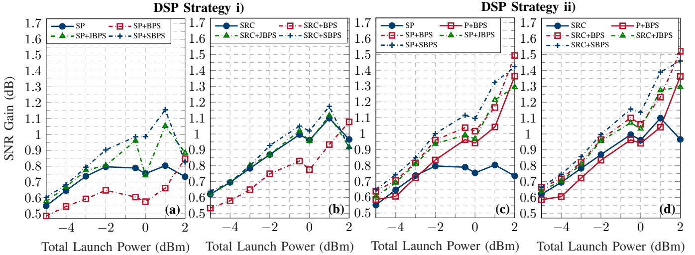
Fig. 10. SNR gain obtained by evolving from single-stage subcarrier-independent pilot-based CPE to joint dual-stage CPE approaches. Results are presented as a function of the total launch power for N_{SC} = 8 , one circulation (432 km) and R_P \approx 2\% , having as first-stage CPE: (a) the SP, (b) the SRC, (c) the SP and LMS prior to the second-stage CPE, and (d) the SRC and LMS prior to the second-stage CPE. Additionally, in (c) and (d), results for the fully subcarrier-independent dual-stage CPE are presented for comparison (P+BPS).
