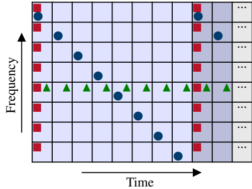
Fig. 1. Frequency/time resource blocks, exemplifying possible allocations for different pilot-based CPE approaches: independent pilots (■), single reference carrier (▲) and spaced pilots (●). Example with N_{\text{SC}} = 8 and R_{\text{P}} = 1/8 (12.5%).
