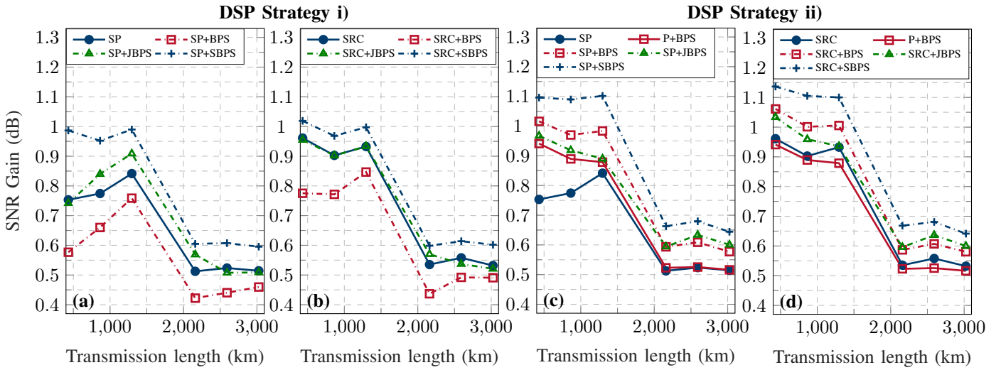
Fig. 11. SNR gain obtained by evolving from single-stage subcarrier-independent pilot-based CPE to joint dual-stage CPE approaches. Results are presented as a function of the transmission distance. And for N_{SC} = 8 , a R_P \approx 2\% and a total launch power of 0 dBm, having as first-stage CPE: (a) the SP, (b) the SRC, (c) the SP and LMS prior to the second-stage CPE, and (d) the SRC and LMS prior to the second-stage CPE. Additionally, in (c) and (d), results for the fully subcarrier-independent dual-stage CPE are presented for comparison (P+BPS).
