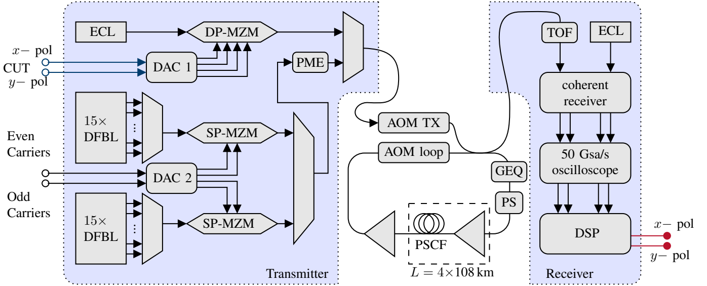
Fig. 4. Experimental setup, as originally presented in [9], utilized to obtain the offline PM-16QAM data (publicly available in an open-access repository [22]), which is hereby reprocessed in this work, employing enhanced joint-subcarrier CPE. In the diagram, we see several building blocks, among which: external cavity laser (ECL), distributed feedback laser (DFBL), digital to analog converter (DAC), dual-pol. (DP-) and single-pol. (SP-) Mach-Zehnder modulator (MZM), polarization multiplexing emulator (PME), acousto-optic modulator (AOM), gain equalizer (GEQ), polarization scrambler (PS), pure silica core fiber (PSCF) and tunable optical filter (TOF)
