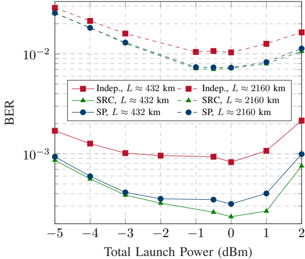
Fig. 7. BER curves as a function of the total launch power for N_{SC} = 8 and R_P \approx 2\% , while using both independent and joint approaches. Results for one circulation (432 km, continuous) and 5 circulations (2160 km, dashed).
