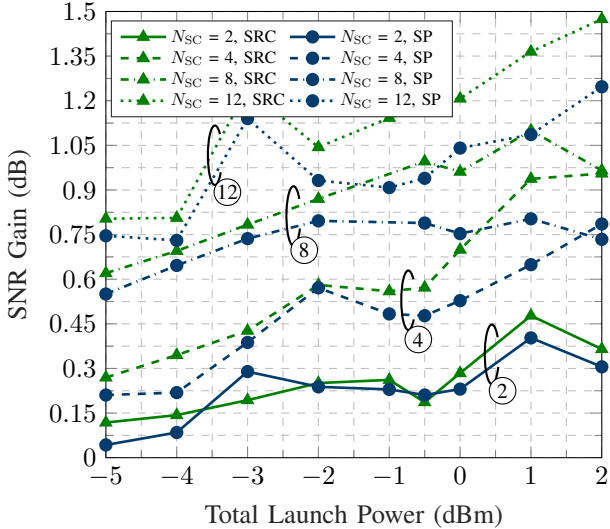
Fig. 6. SNR gain obtained by evolving from subcarrier-independent to joint pilot-based CPE approaches. Results are displayed as a function of the total launch power. R_P \approx 2\% and L = 432 km were used.
