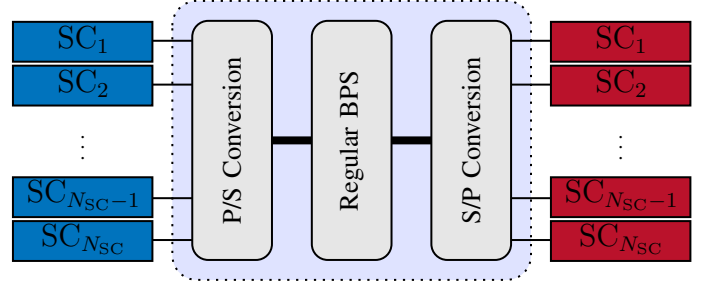
Fig. 3. Demonstrative diagram of the implementation of serialized BPS (SBPS). In this method, the LPN compensation is implicitly performed in the BPS block, prior to the serial-to-parallel conversion.
