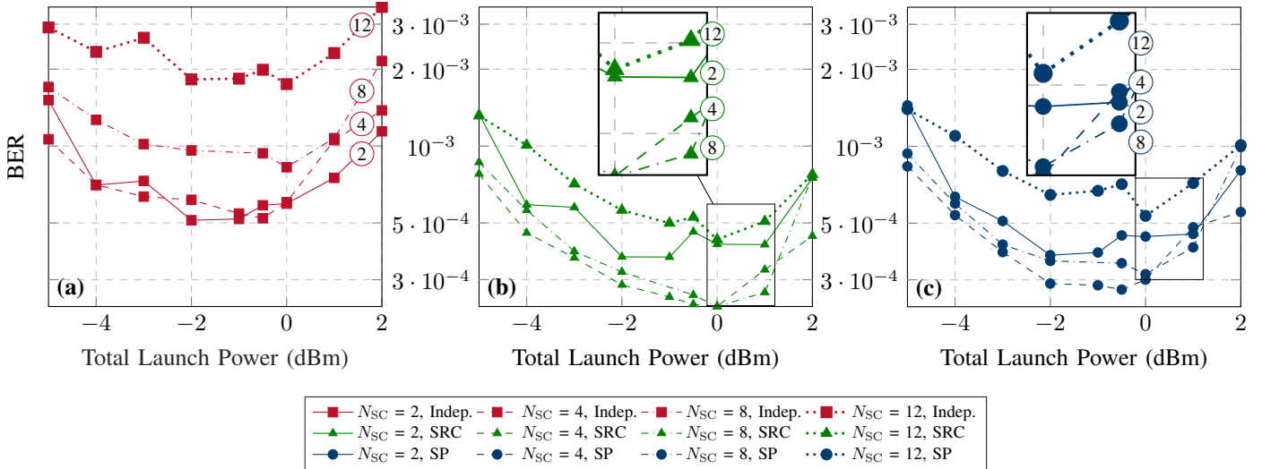
Fig. 5. BER curves as a function of the total launch power for N_{SC}=2, 4, 8, and 12 , one circulation (432 km), and R_P \approx 2\% , while using (a) subcarrier-independent pilot-based CPE, or joint-subcarrier pilot-based CPE, be it (b) SRC or (c) SP.
