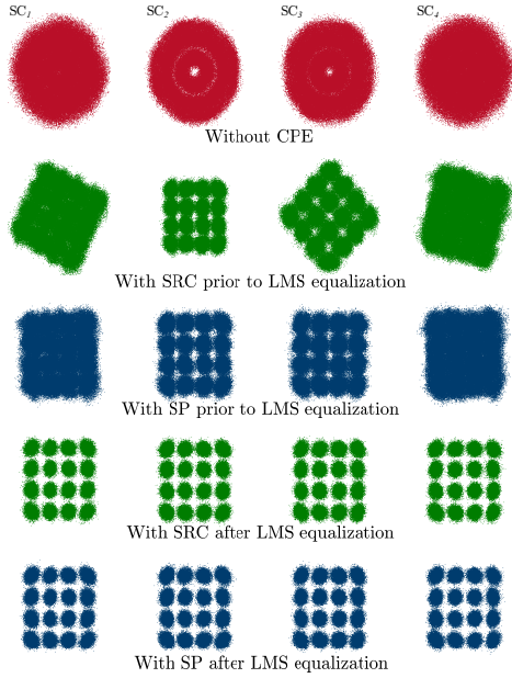
Fig. 9. Constellations after the coarse CMA equalization, before and after the joint-subcarrier pilot-based CPE stage, and also after LMS equalization. Results for R_P \approx 2\% , N_{SC} = 4 , a launch power of 0 dBm and L = 432 km.
