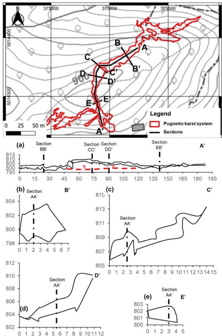
FIGURE 6 Longitudinal and transversal sections along Borna Maggiore Cave (CRS: WGS84/UTM zone 32N – EPSG 32632). Horizontal and vertical distances are in meters.
