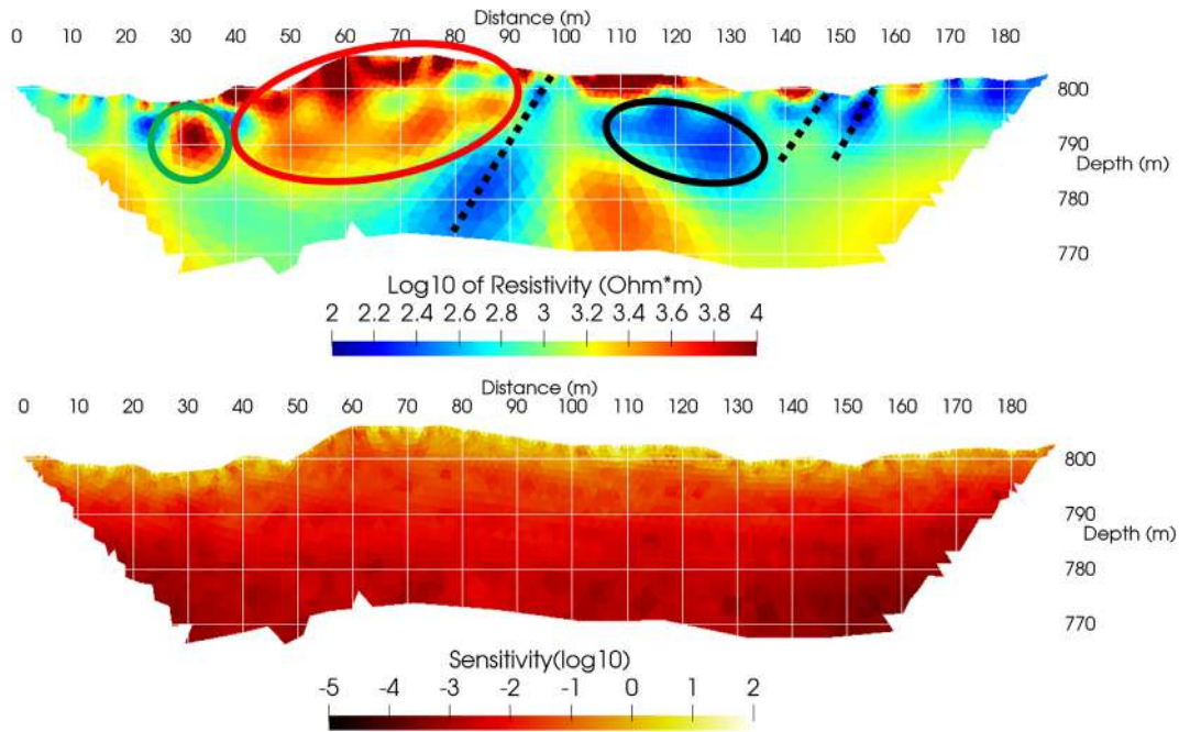
FIGURE 9 2D resistivity model (top) and sensitivity map (bottom) of the rock mass below the cave after 2D inversions. The first electrode, nearest to the cave entrance, is in the left part of the picture.
