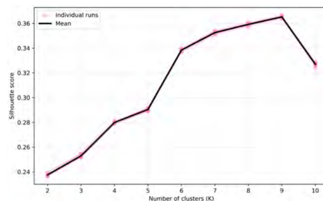
Figure 5. Silhouette scores across candidate cluster numbers ( K ) under repeated K-means subsampling. Faint lines show individual runs; the black line shows the mean score across repetitions.
