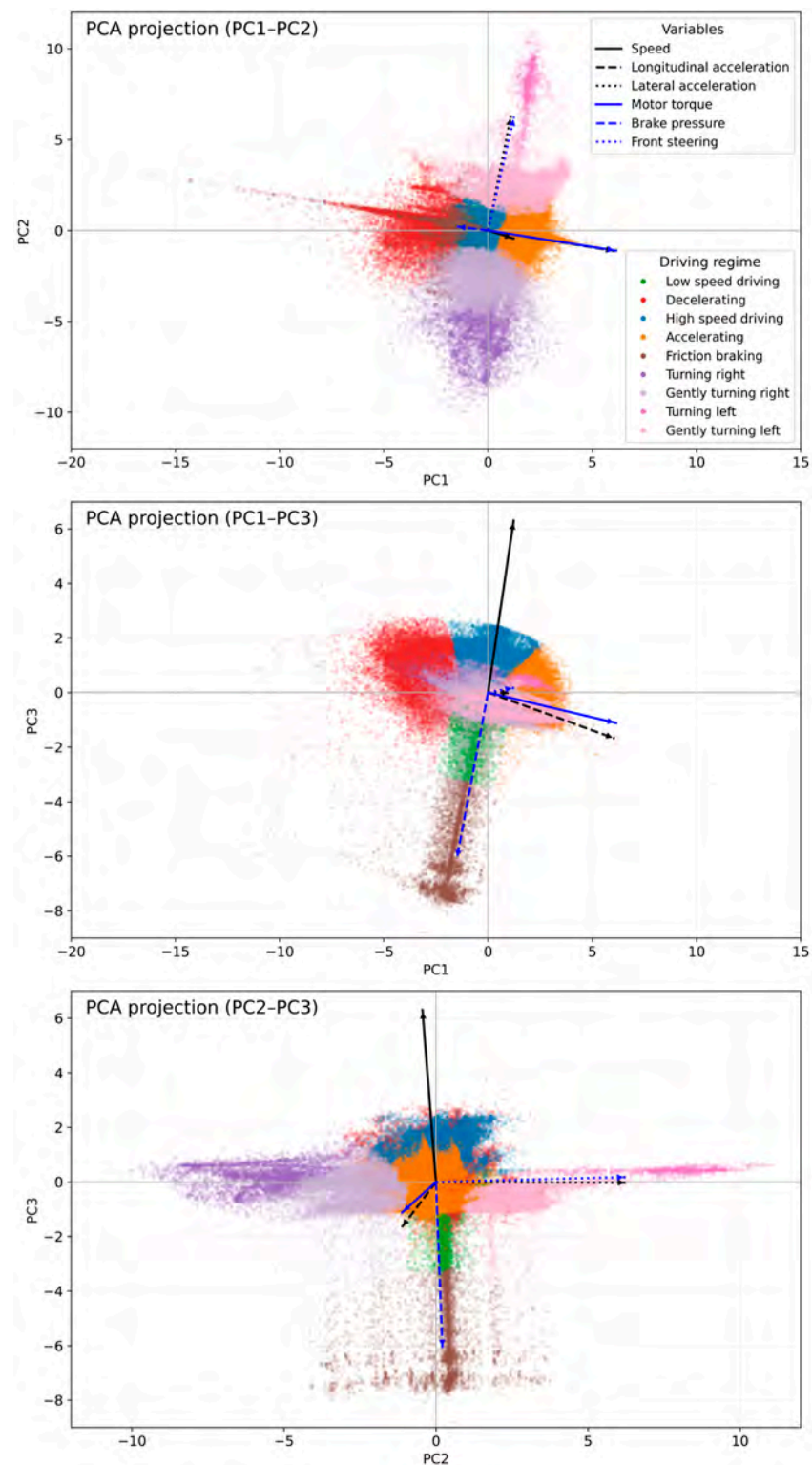
Figure 7. Principal component analysis (PCA) projections of the retained nine-cluster driving-context solution in the PC1–PC2, PC1–PC3, and PC2–PC3 planes, with loading vectors overlaid.
