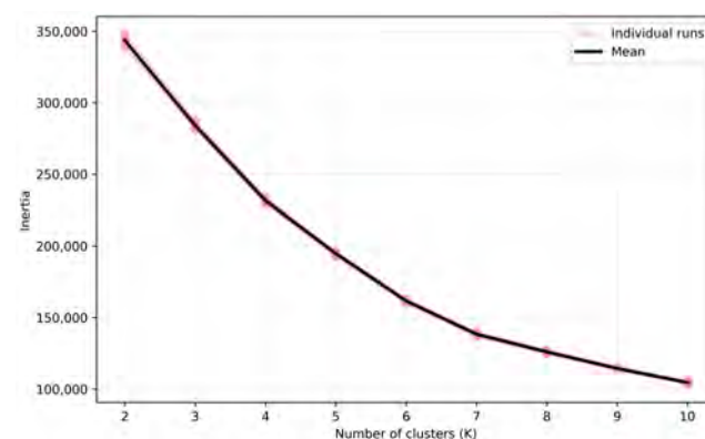
Figure 6. Inertia across candidate cluster numbers ( K ) under repeated K-means subsampling. Faint lines show individual runs; the black line shows the mean across repetitions.
