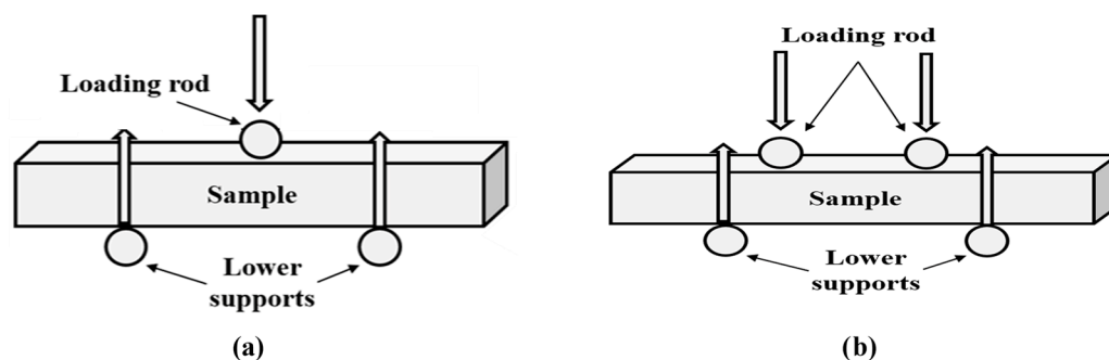
Figure 16. Schematic of the working principle of the (a) three-point and (b) four-point bending tests.
