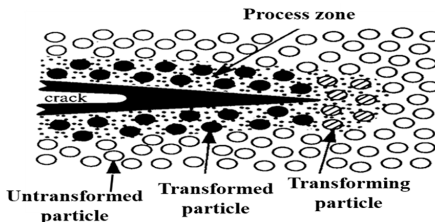
Figure 3. Schematic view of transformation toughening process. Reproduced with permission from Ref. [23], Copyright 1999 Elsevier.
