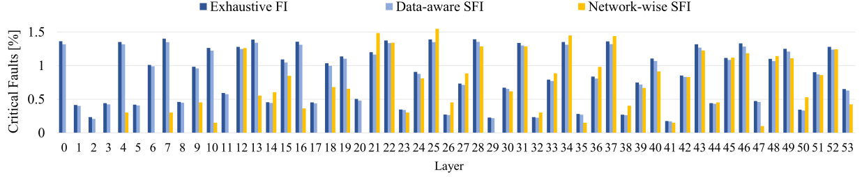
Fig. 7: MobileNetV2: a data-aware SFI yields statistically significant results, and correctly depicts the per-layer criticality.
