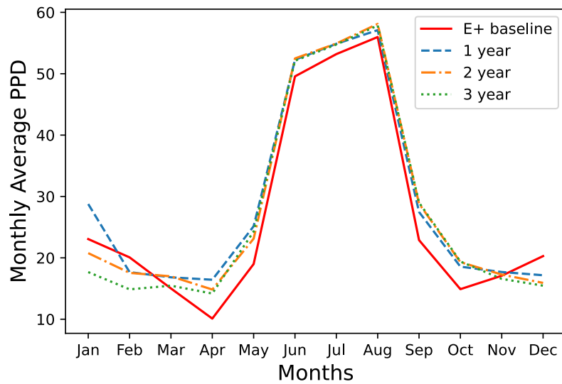
Fig. 5. Three years comparison between the EnergyPlus (E+) baseline and the proposed approach with Imitation Learning pretraining, in terms of monthly average PPD.
