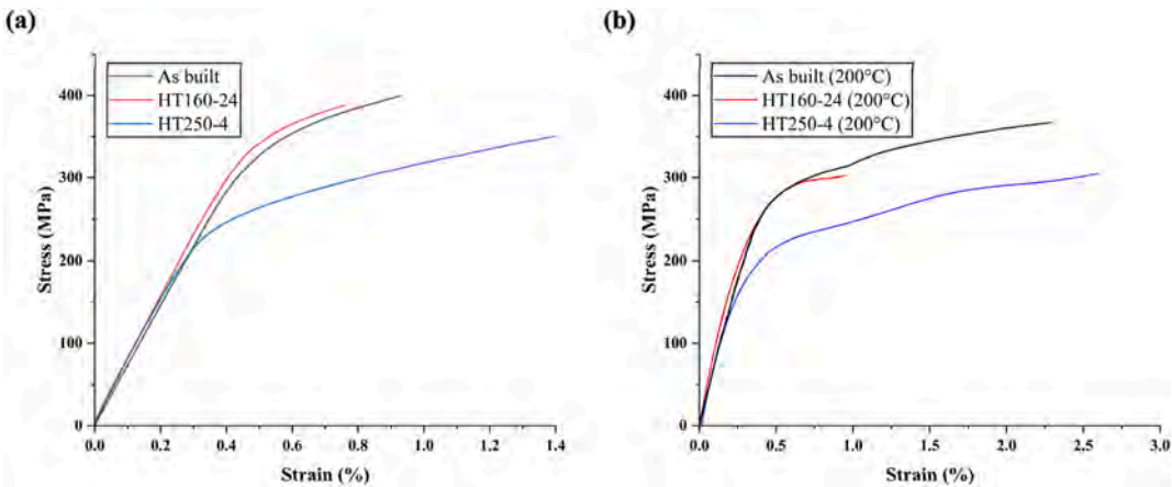
Figure 12. Representative engineering stress–strain curves of the PBF-LB/M AlSi10Cu8Mg alloy under different aging treatments. (a) Room-temperature tensile response, and (b) Elevated-temperature tensile behavior at 200 °C.
