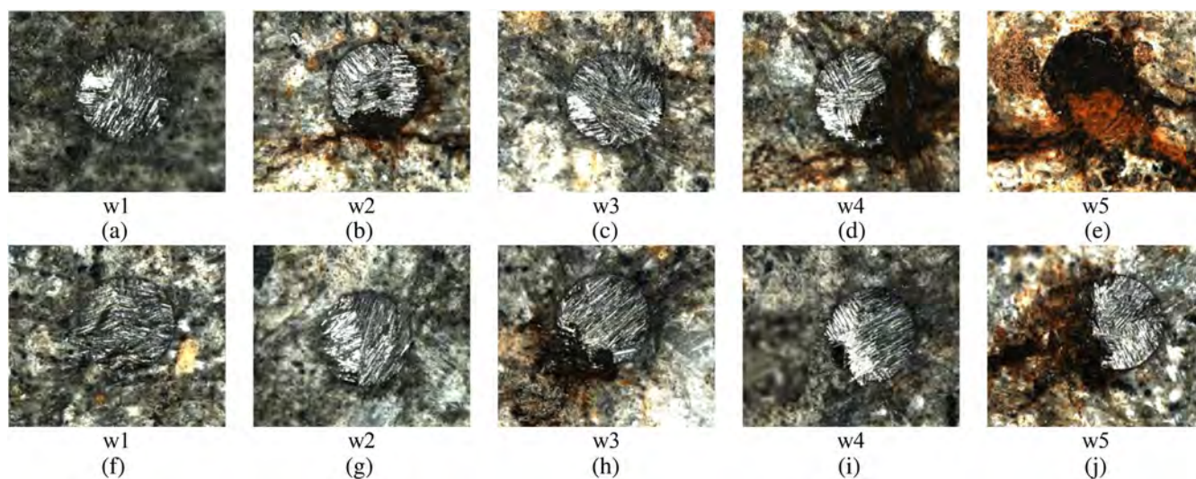
FIGURE 17 Photographic acquisitions of the corrosion state of wires of sample Aged_02 (a–e) and the painted and aged sample (f–j), by means of the optical microscope (magnification 5×).
