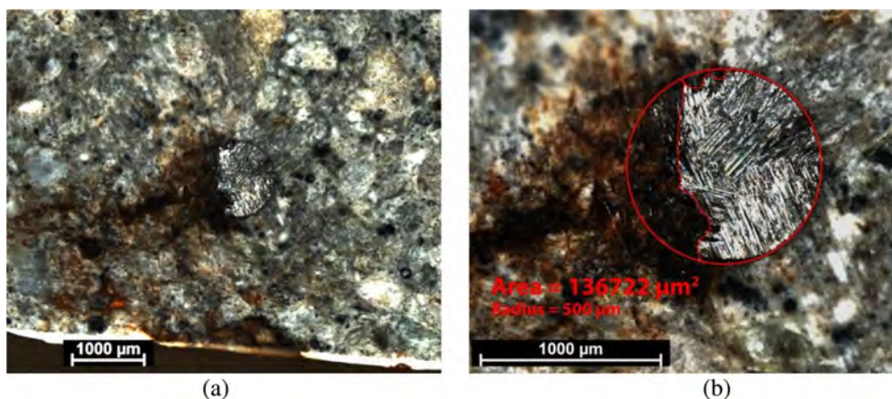
FIGURE 18 Magnification of wire w5 of the sample presenting a layer of paint (painted and aged), magnification 2× (a) and 5× reporting the radius of the wire and the measured loss of area due to corrosion (b), respectively.
