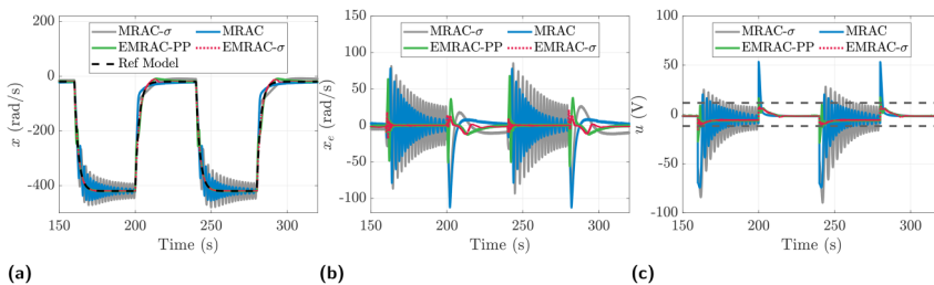
Figure 13. Experimental results for the S7 reference signal for the MRAC (blue line), MRAC- \sigma (gray line), EMRAC-PP (green line) and EMRAC- \sigma (red line) strategies: (a) speed and reference speed (dashed black line), (b) tracking error, and (c) control action generated by the controller along with the saturation limits (dark gray dashed lines).
