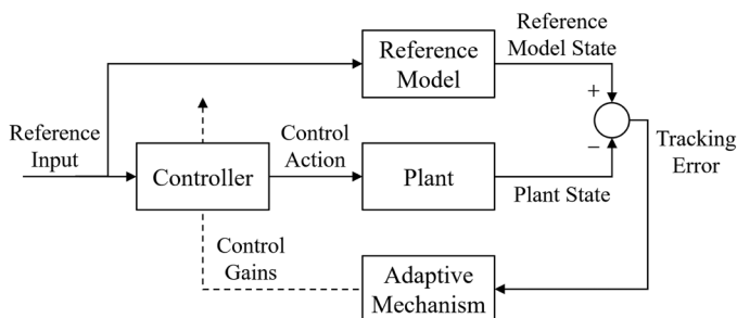
Figure 1. Block diagram of a typical MRAC algorithm.
