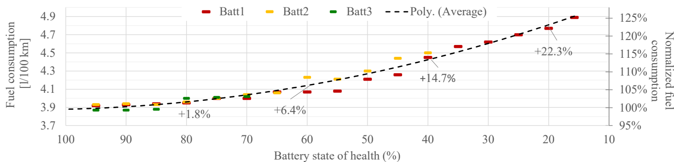
Fig. 5 HEV fuel economy capability predicted by DP in the WLTP over retained battery SOH values for the three test cases and related average.
