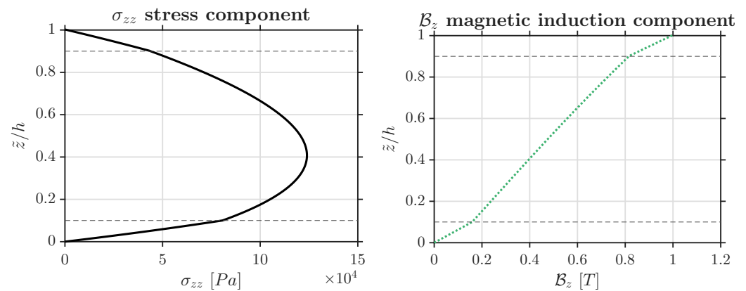
Figure 9. NC4: simply-supported sandwich Adaptive Wood/Soft Adaptive Wood/Adaptive Wood spherical shell considering LB2 Load Boundary conditions ( \mathcal{B}_{z_t} = 1 T, \mathcal{B}_{z_b} = 0 T and \theta_t = 1.5 K, \theta_b = 0 K). Thickness ratio is R_\alpha/h = 10 . Results are obtained via the 3D-u- \theta - \psi model.
