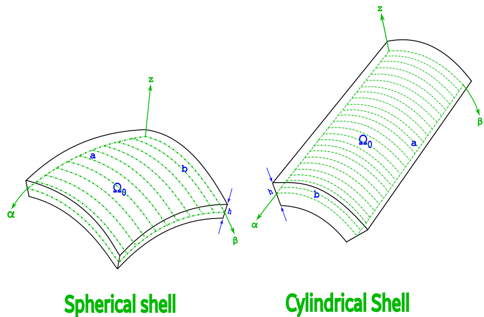
Figure 1. Geometries, mixed curvilinear orthogonal reference system and middle reference surface for Preliminary Assessments (PA) and New Cases (NC). Dotted lines represent the middle reference surface \Omega_0 . The mixed curvilinear orthogonal reference system is visible for each structure.
