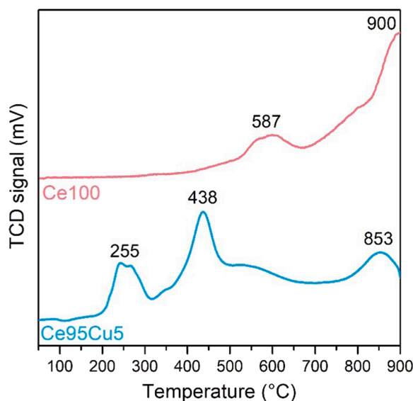
Fig. 3. \text{H}_2 -TPR profiles of the two catalysts.
