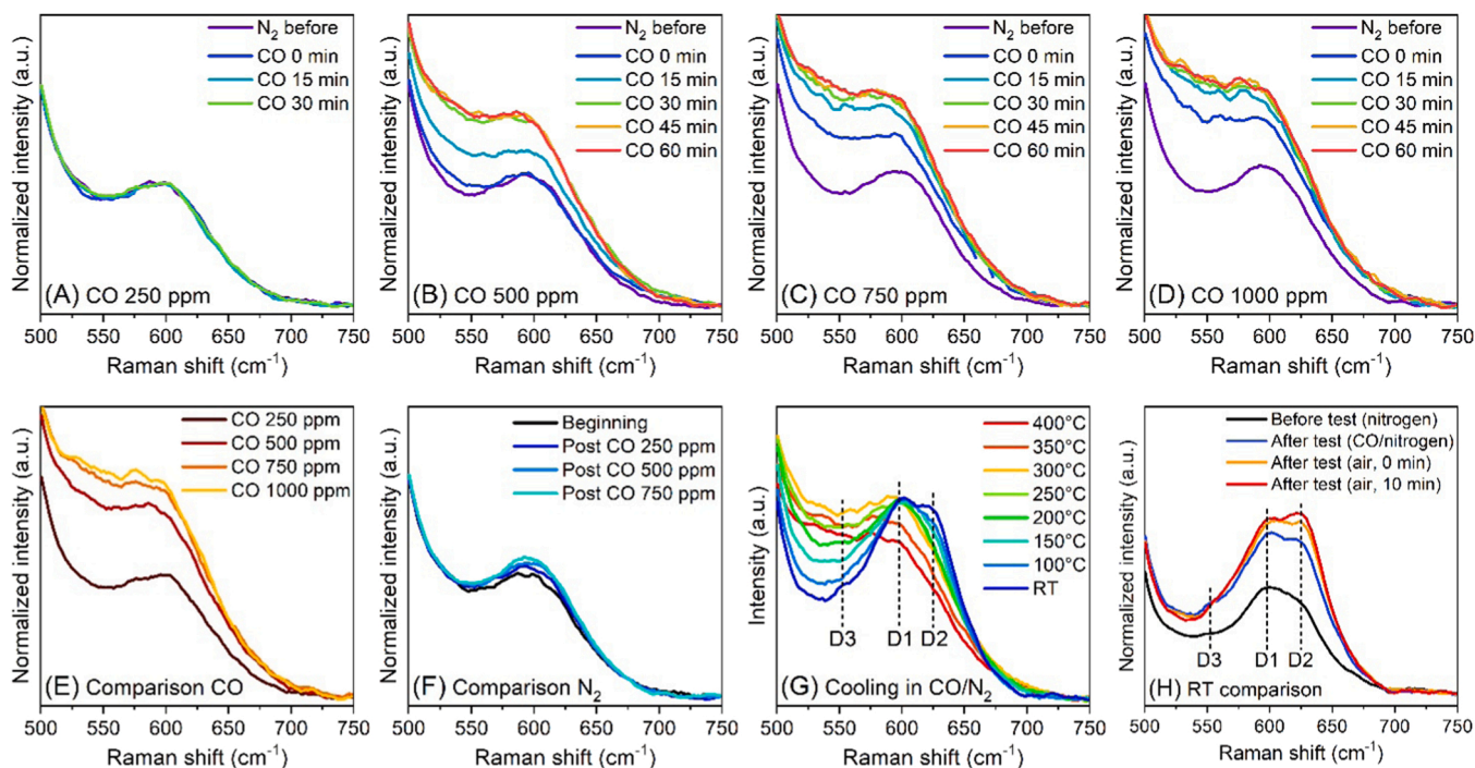
Fig. 8. Magnification of the defect band in in situ Raman spectra collected on the Ce95Cu5 sample in different conditions. Spectra acquired at 400 °C over time while flowing a mixture containing 250 ppm (A), 500 ppm (B), 750 ppm (C), or 1000 ppm (D) of CO in N 2 . Comparison of the spectra recorded at 400 °C after 60 min of exposure to different concentrations of CO (E). Comparison of the spectra collected at 400 °C while flushing the cell with pure N 2 before and after exposure to different concentrations of CO (F). Spectra acquired at different temperatures while cooling down the sample after the test, under an atmosphere of 1000 ppm of CO in N 2 (G). Comparison of the spectra collected at RT in different atmospheres before and after the test (H).
