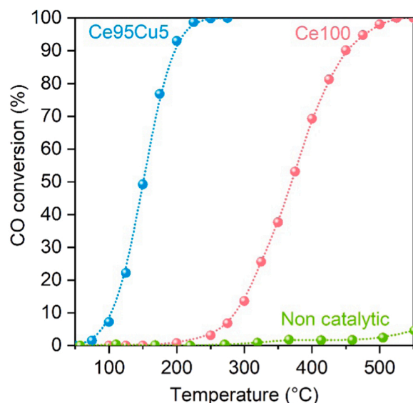
Fig. 6. Light-off curves reporting the percentage of CO converted as a function of the temperature during CO oxidation tests (feed gas mixture containing 1000 ppm of CO and 10% of \text{O}_2 in \text{N}_2 , temperature increased step by step). Results are similar to those of analogous hydrothermally-synthesized samples described in [30].
