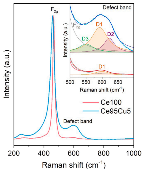
Fig. 4. Raman spectra of the two catalysts collected at RT, normalized to the \text{F}_{2g} peak intensity. In the inset, the defect band is magnified, highlighting the different deconvoluted peaks (thin lines).
