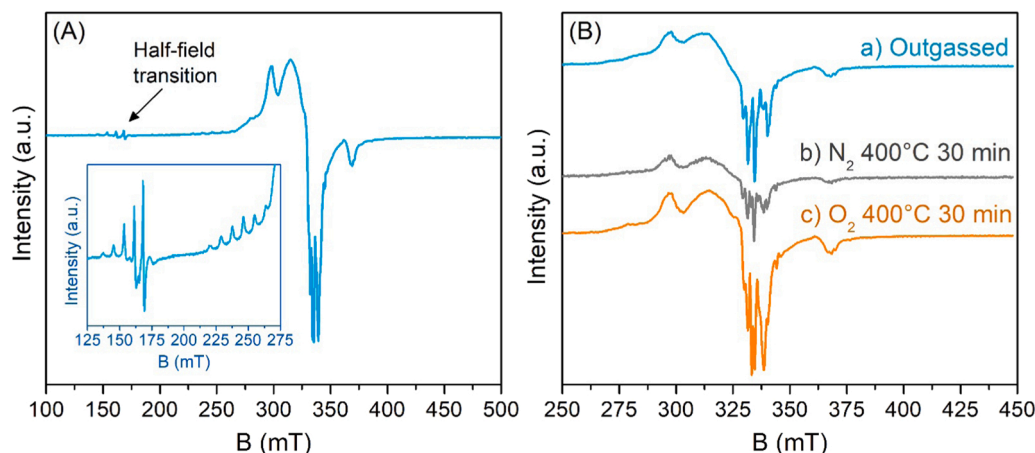
Fig. 2. Complete EPR spectrum of the Ce95Cu5 sample acquired at -196^{\circ}\text{C} after outgassing the powder (A); in the inset, the half-field transition region is magnified. EPR spectra collected at -196^{\circ}\text{C} after treating the Ce95Cu5 catalyst in different ways (B): after outgassing the sample (a), after thermal treatment in \text{N}_2 at 400^{\circ}\text{C} for 30 min (b), and after thermal treatment in \text{O}_2 at 400^{\circ}\text{C} for 30 min (c).
