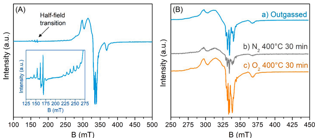
Fig. 2. Complete EPR spectrum of the Ce95Cu5 sample acquired at -196\text{ }^{\circ}\text{C} after outgassing the powder (A); in the inset, the half-field transition region is magnified. EPR spectra collected at -196\text{ }^{\circ}\text{C} after treating the Ce95Cu5 catalyst in different ways (B): after outgassing the sample (a), after thermal treatment in \text{N}_2 at 400\text{ }^{\circ}\text{C} for 30 min (b), and after thermal treatment in \text{O}_2 at 400\text{ }^{\circ}\text{C} for 30 min (c).
