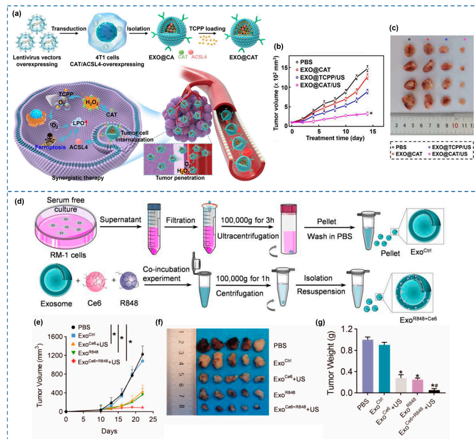
Figure 5. (a) Schematic illustration of the preparation EXO@CAT NVs and treatment mechanism based on tumor vessel extravasation, tumor penetration, and cell internalization, followed by SDT and ferroptosis. (b) Tumor growth curves among all treatment groups. * p < 0.05 . (c) Representative pictures of explanted tumors. Reproduced with permission from [30]. (d) Scheme of the fabrication of Exo Ce6 R848 and control counterpart. (e) Mean tumor growth curve of primary tumors subjected to the treatments. * p < 0.05 . (f) Digital photo of the explanted tumors. (g) Weights of the explanted tumors. * p < 0.05 , # p < 0.05 . Reproduced with permission from [157].
