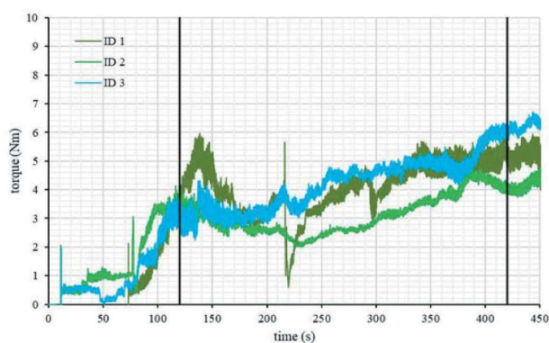
Figure 14. Torque over time graph for dynamic adhesion tests.
