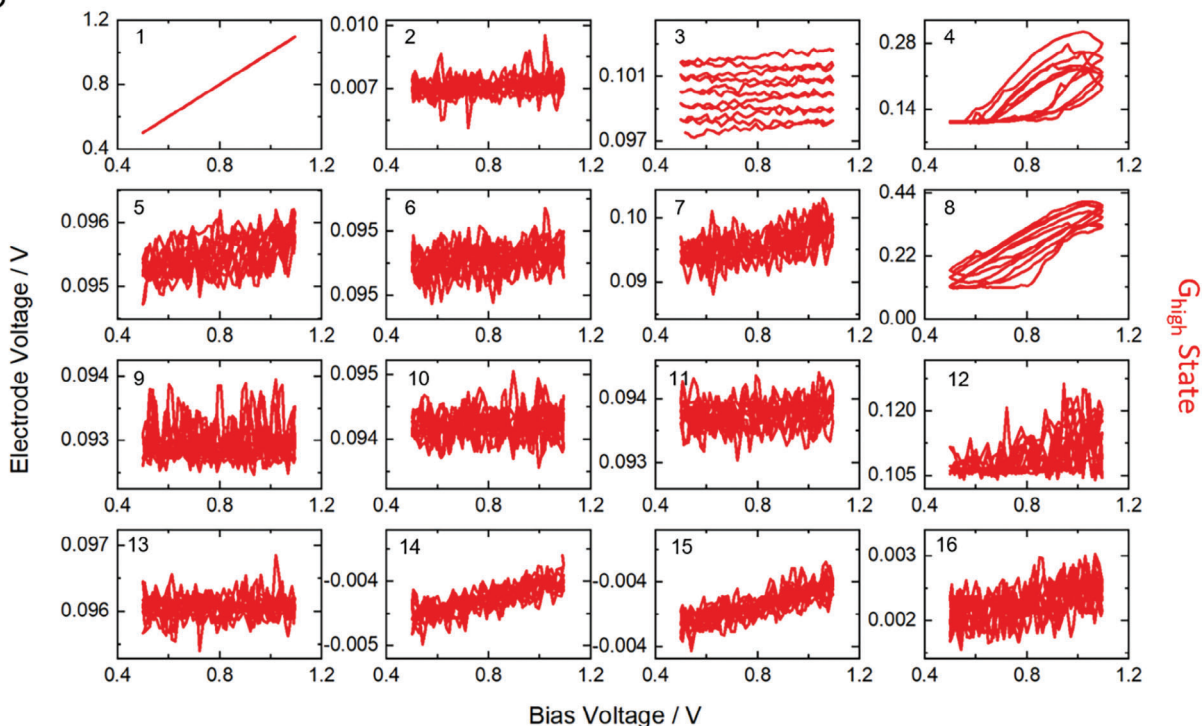
Figure 5. Lissajous analysis of the nonlinear response of each electrode. a) Lissajous analysis before activation ( G_{\text{low}} state). b) Lissajous analysis after activation ( G_{\text{high}} state).
