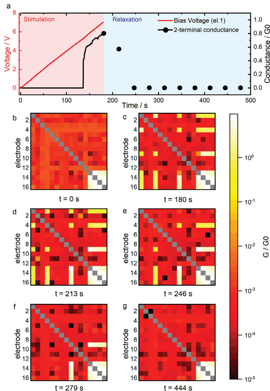
Figure 2. Conductance matrix analysis. a) I - V ramp characterization showing potentialiation and spontaneous relaxation over time. b) Pristine state conductance matrix. c) Conductance matrix after network potentiation. d-g) Conductance matrix analysis of the network relaxation over time.
