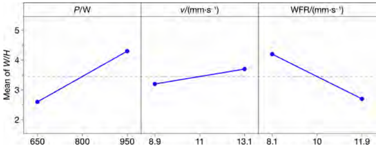
Figure 12 W/H main effects factorial plot (see online version for colours)
