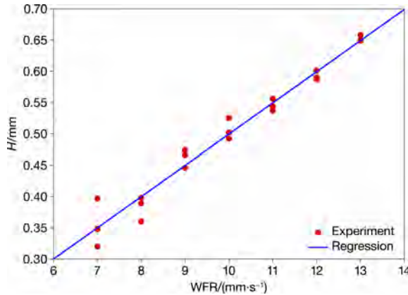
Figure 7 H versus WFR regression model (see online version for colours)
