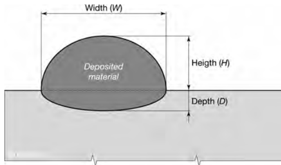
Figure 4 Geometrical features of the melt pool; depth ( D ), width ( W ), height ( H )
