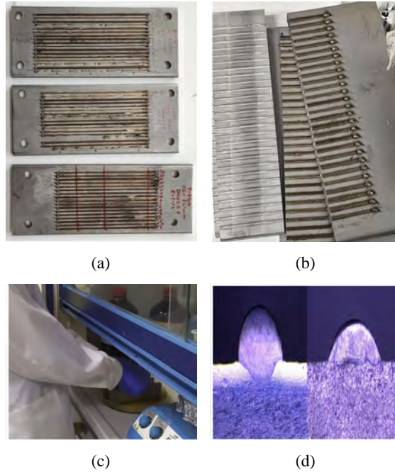
Figure 6 Extraction of W , H , D , dimensions, (a) single tracks, (b) sections to be polished, (c) etching with hydrochloric acid, (d) measurements with microscope (see online version for colours)
