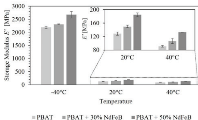
Figure 6. Plot of the Storage Modulus at different temperatures for the pure polymer and the composites. For better visualization, the inset shows a zoomed view of the 20 and 40 °C values of the Storage Modulus for the different compositions.
