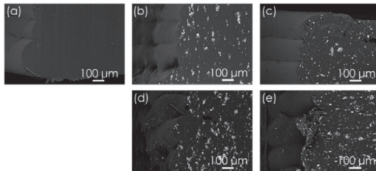
Figure 5. SEM images of pure PBAT (a), PBAT + 30% NdFeB printed respectively with (b) and without (c) the magnet support, and PBAT + 50% NdFeB printed respectively with (d) and without (e) the support magnet
