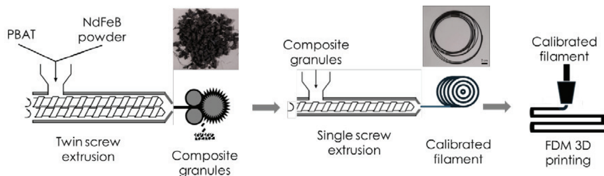
Figure 2 Experimental set-up to produce composite granules and calibrated filaments
