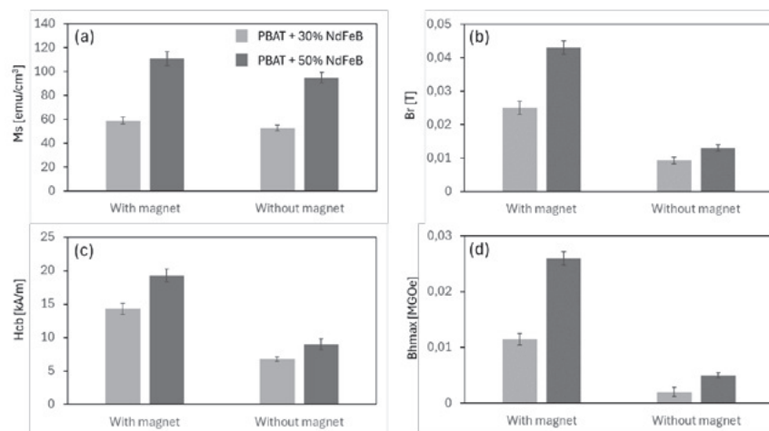
Figure 7. The values of M_s , B_r , H_{cb} , BH_{max} determined by VSM measurements
