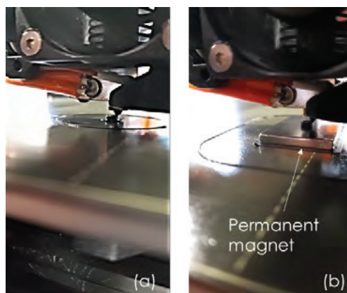
Figure 3 FDM 3D printing of magnetic composite without (a) and with the aid of a permanent magnet
