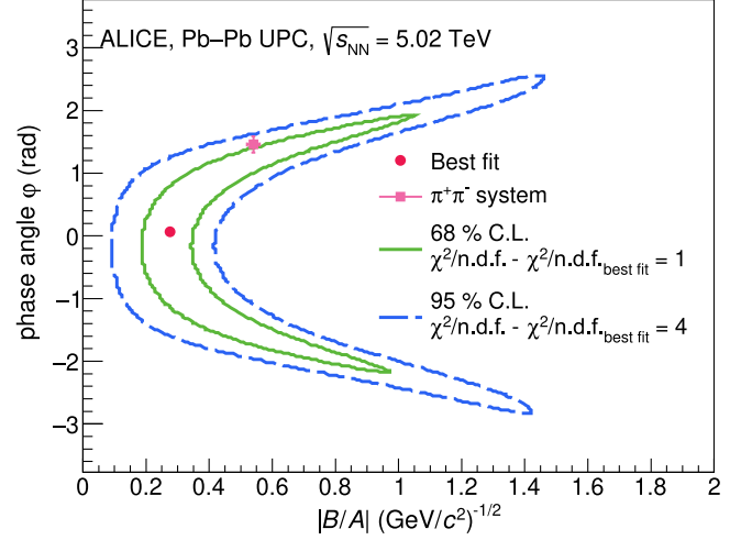
FIG. 3. Confidence regions for the relative fraction of direct K^+K^- contribution with respect to the amplitude of \phi(1020) \rightarrow K^+K^- ( |B_{KK}/A_\phi| ) and the relative phase angle between \phi(1020) \rightarrow K^+K^- and direct K^+K^- ( \varphi ). The best fit is shown as a red dot at |B_{KK}/A_\phi| = 0.28 (\text{GeV}/c^2)^{-1/2} and \varphi = 0.06 rad found with \chi^2/\text{n.d.f.}_{\text{best fit}} = 0.3 , while a pink square at the |B_{\pi\pi}/A_\rho| = 0.54 \pm 0.01(\text{stat}) \pm 0.02(\text{syst}) (\text{GeV}/c^2)^{-1/2} [23] and relative phase angle \varphi = 1.46 \pm 0.11(\text{stat}) \pm 0.07(\text{syst}) rad [22] indicates the best-fit values for \rho plus direct \pi^+\pi^- . The green solid line and blue dashed line represent the boundary of 68% and 95% confidence regions, respectively.
