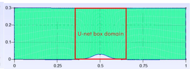
Figure 5 : Bump - high fidelity mesh (30k nodes)
