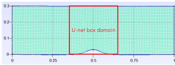
Figure 4 : Bump - low fidelity mesh (3k nodes)
