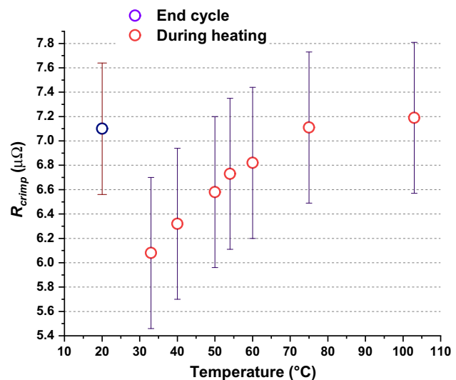
Fig. 12 Comparison of the R_{crimp} measurements. (These resistance values were reported at 20 °C taking into account the temperature coefficient of the lug material to be comparable with the resistance values measured before the cycle and after the cooling times (at 20 °C).) respectively at the end of the thermal cycle (blue dot) and during the heating period (red dots) in the thermal cycle I. These measurements were respectively made with the micro-ohmmeter and with the voltammeter method
