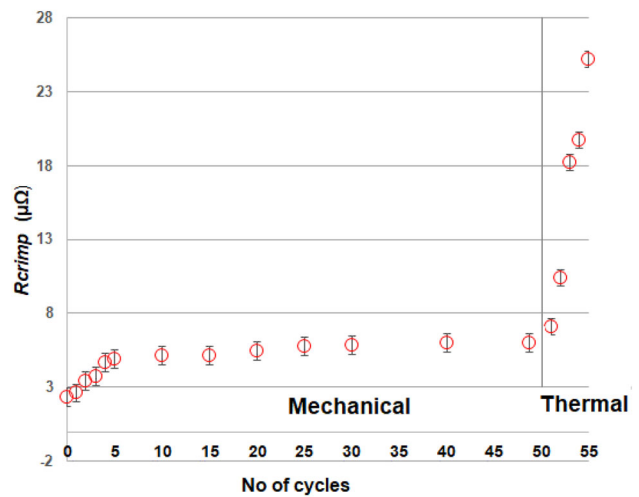
Fig. 11 R_{crimp} of lug 1 submitted first to mechanical stresses (the first fifty in Fig. 10) and after to thermal ones (last five)
