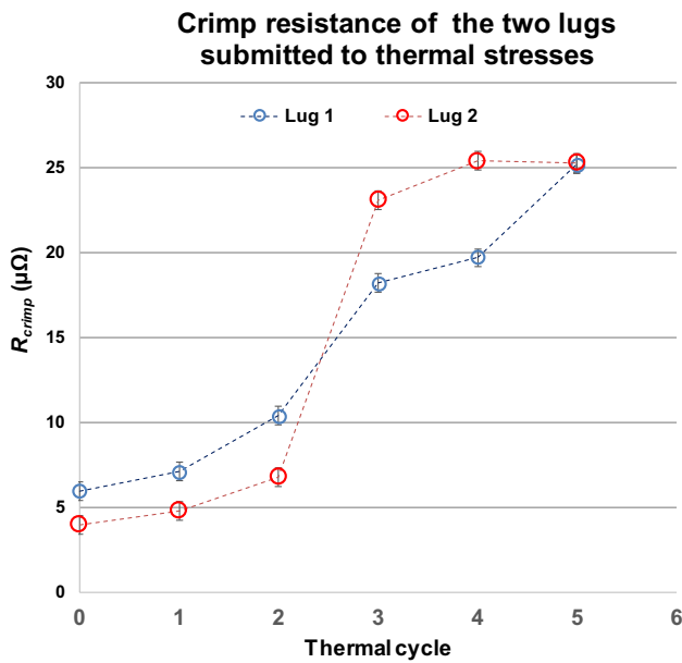
Fig. 10 Trend of the R_{crimp} values of the two lugs after each thermal cycle
