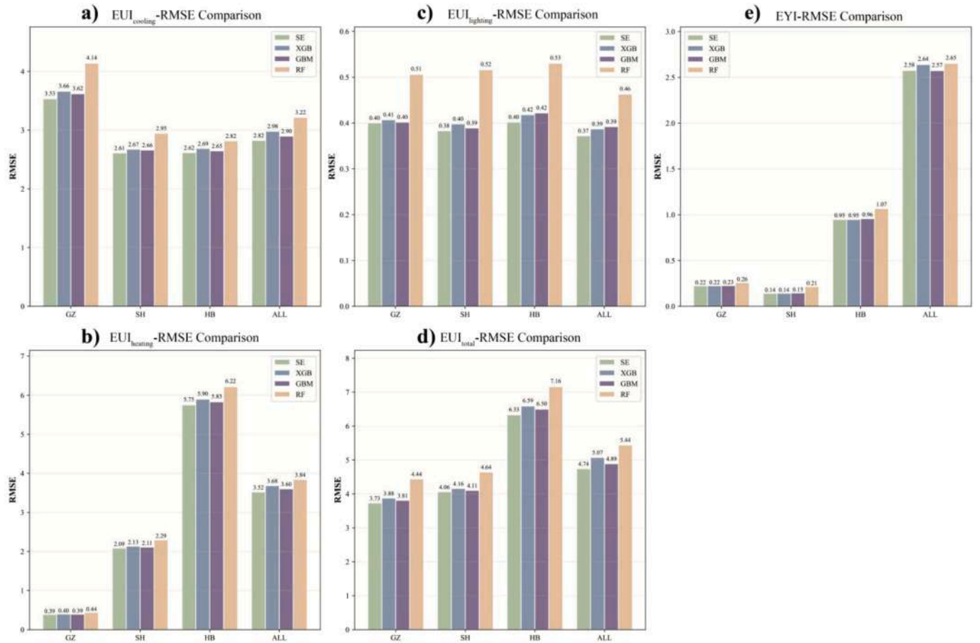
Fig. 7. RMSE Comparison between different models (Validation frame).
