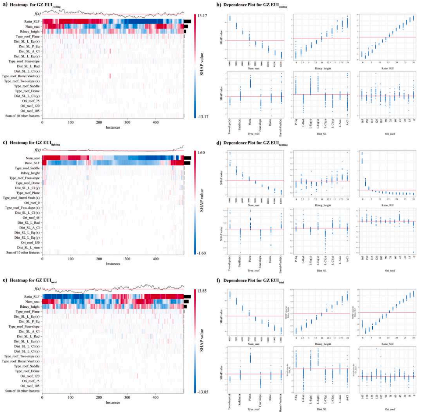
Fig. 10. Typical feature attribution analysis for GZ.
