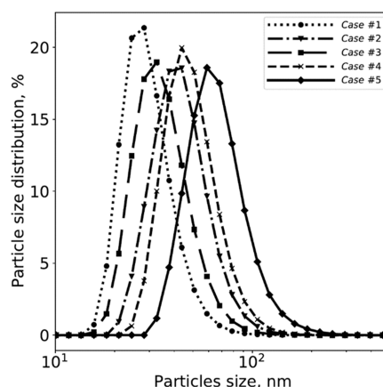
Figure 1. \text{Mg}(\text{OH})_2 PSDs for Cases #1–5. PSDs were obtained after 5 min of ultrasound treatment and using PAA as a dispersant. Measurements were carried out using the Malvern Zetasizer Nano ZSP.
