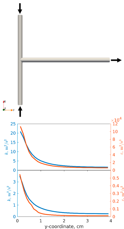
Figure 4. Spatial evolution of TDR, \epsilon , (red line) and kinetic energy, k , (blue line) over the mixing channel length. Case study operative conditions: T_{2mm} -mixer, 12.3 m/s velocity in the mixing channel namely flow rate of cases #1–5 (top). T_{2mm} -mixer, 4.1 m/s velocity in the mixing channel, namely the flow rate of case #7 (bottom).
