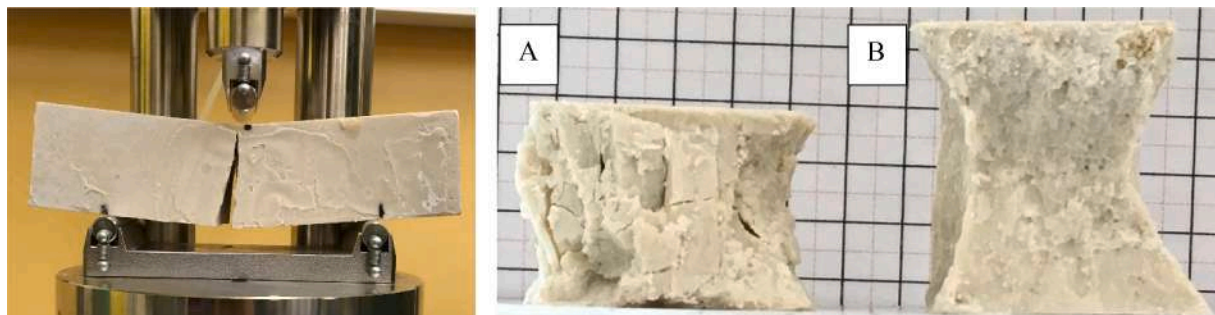
Fig. 15. Example of failure mode of samples tested at long curing time. On the left: failure of s sample during a tensile strength assessment. On the right: two different failure modes of samples after a UCS test: an irregular shape (A) and an hourglass shape (B).
