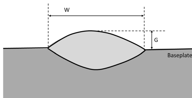
Fig. 2 Geometrical features of the SSTs melt pools. G and W respectively indicate the growth and the width of a melt pool
