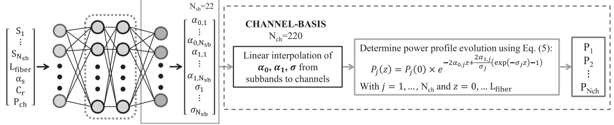
Fig. 2. Testing process from subbands to channels for (a) ANN Model 1 and (b) ANN Model 2. For Model 1, the loss profiles L , the input power loads S and the output power profiles P are in logarithmic units.
