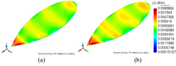
Fig. 5. Current distribution of the NASA almond model from. (a) Mixed NESA (b) The iterative solution.
