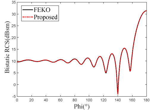
Fig. 4. Bistatic RCS of the PEC sphere.
