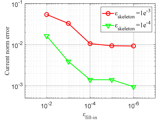
Fig. 3. The current norm error compared to the brute force LU factorization with different tolerance.
