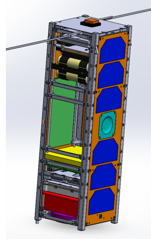
Fig. 9: ELECTRA spacecraft
