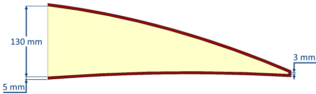
Figure 2: Morphing trailing edge structure
