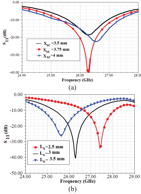
Fig. 4: Reflection coefficient for various values of (a) X_{SC} , L_s = 3\text{mm} , W_s = 0.5\text{mm} , dd = 0\text{mm} , tt = 2.2\text{mm} . (b) Slot length, L_s , X_{SC} = 3.75\text{mm} , W_s = 0.5\text{mm} , dd = 0\text{mm} , tt = 2.2\text{mm} .
