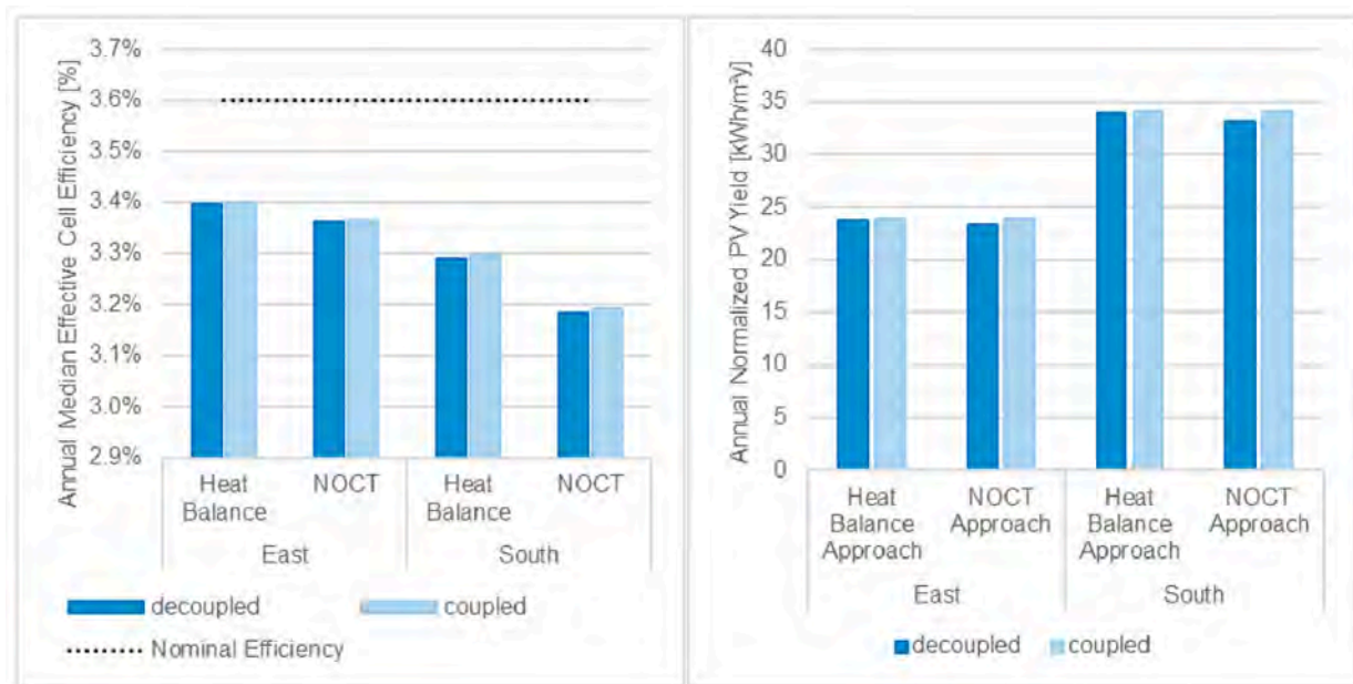
Figure 20. STPV effective efficiency and PV yield for heat-balance and NOCT cell-temperature assessment approaches under decoupled and coupled formulations: (Left) annual median effective efficiency compared with nominal efficiency; (Right) annual normalized PV yield.
