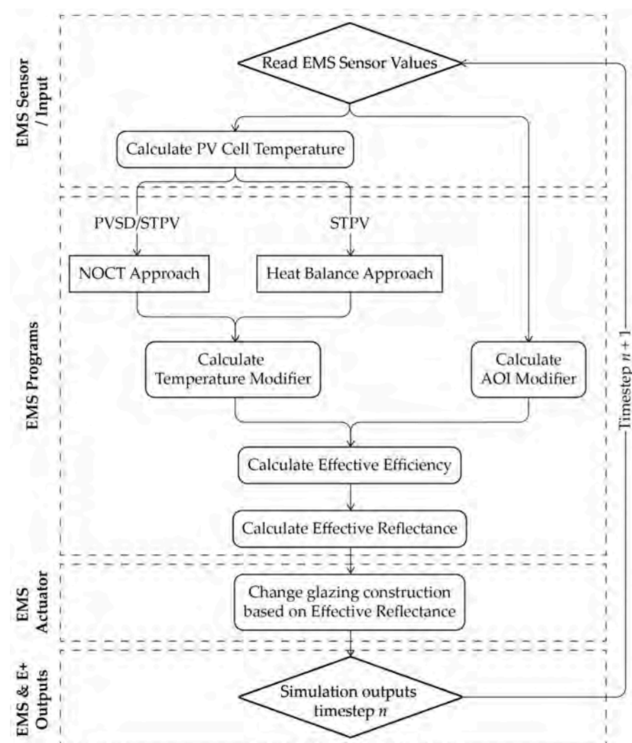
Figure 12. EnergyPlus EMS scheme for the STPV coupled formulation with effective-efficiency-based construction switching.
