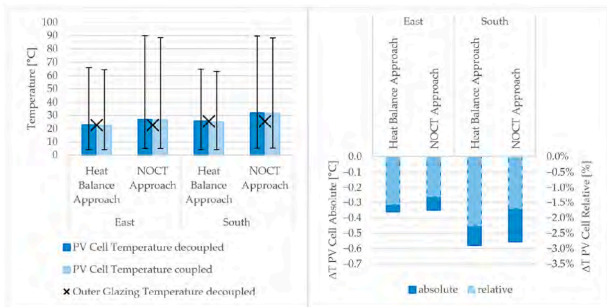
Figure 19. STPV cell-temperature assessment under coupled and decoupled formulations: (Left) annual median PV cell temperature during sunlit hours for heat-balance and NOCT approaches; (Right) absolute and relative PV cell-temperature differences between coupled and decoupled formulations.
