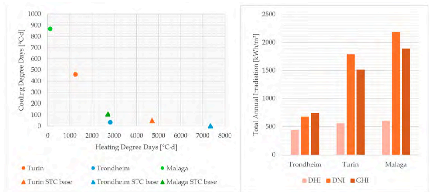
Figure 8. Degree-day and annual irradiation comparison for the reference climate and additional climate-transferability locations.
