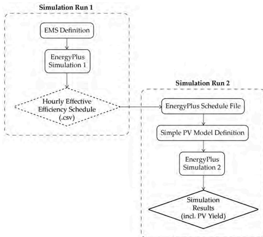
Figure 6. Two-run EnergyPlus sequence for generating the hourly effective-efficiency schedule and applying it in the Simple PV model.
