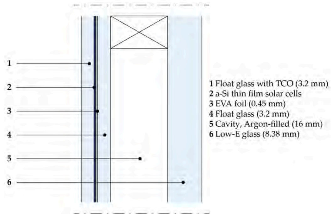
Figure 3. STPV glazing stratigraphy used for the modeling-choice analysis, with the STPV laminate as the exterior-facing layer of the double-glazing unit.
