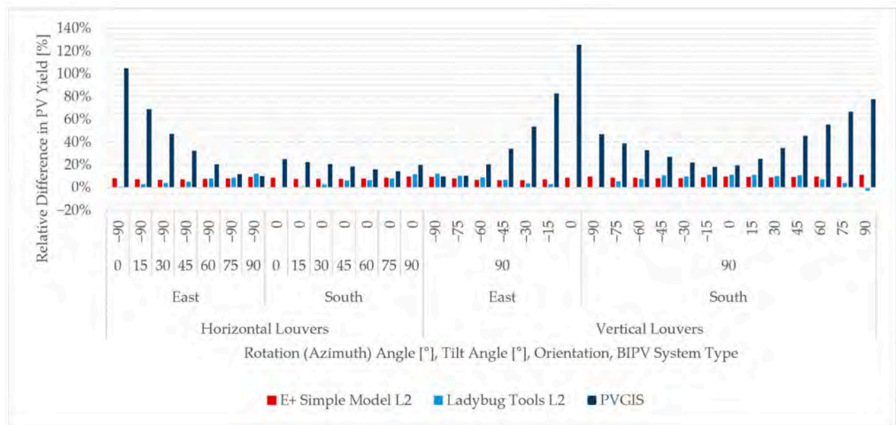
Figure 16. Relative differences in annual PV yield across assessment approaches for Level 2 PVSD configurations.
