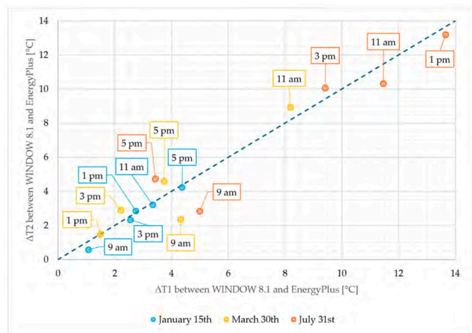
Figure A3. Cross-tool temperature differences for the exterior STPV laminate surface nodes: T1/\theta_1 on the x-Axis and T2/\theta_2 on the y-Axis. The dashed line indicates equal cross-tool differences.
