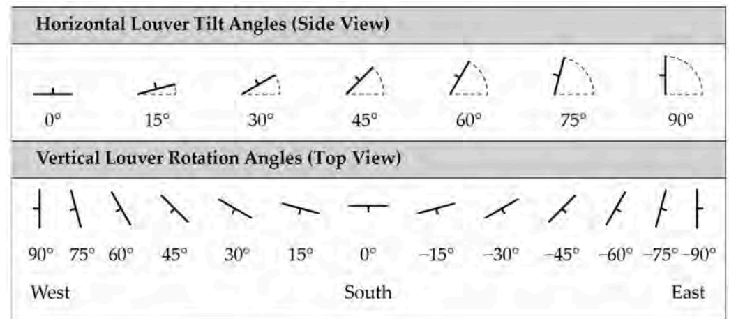
Figure 9. PVGIS-based angle conventions used to report PVSD configurations: horizontal louver tilt angles in side view and vertical louver rotation angles in top view.
