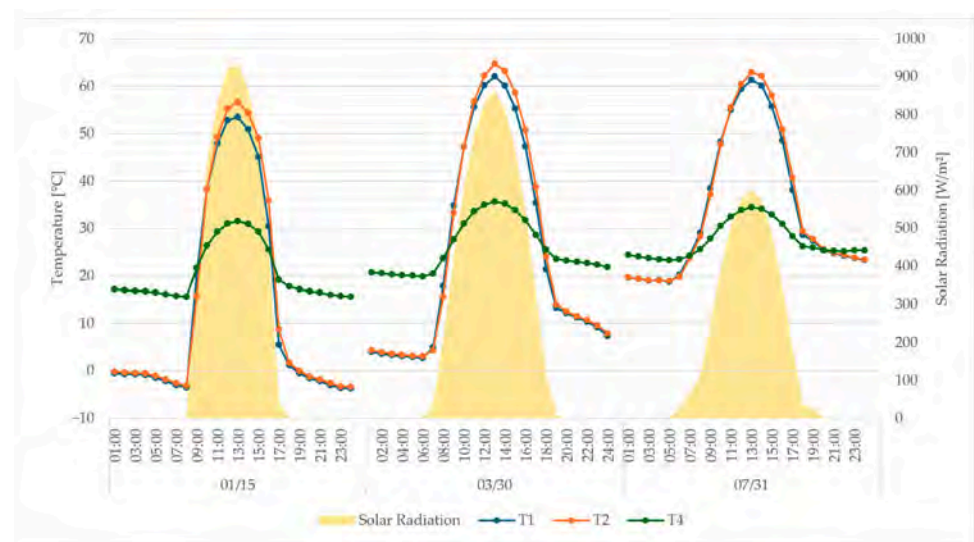
Figure A1. Selected EnergyPlus boundary conditions and glazing temperatures used for the STPV temperature-reconstruction verification check.
