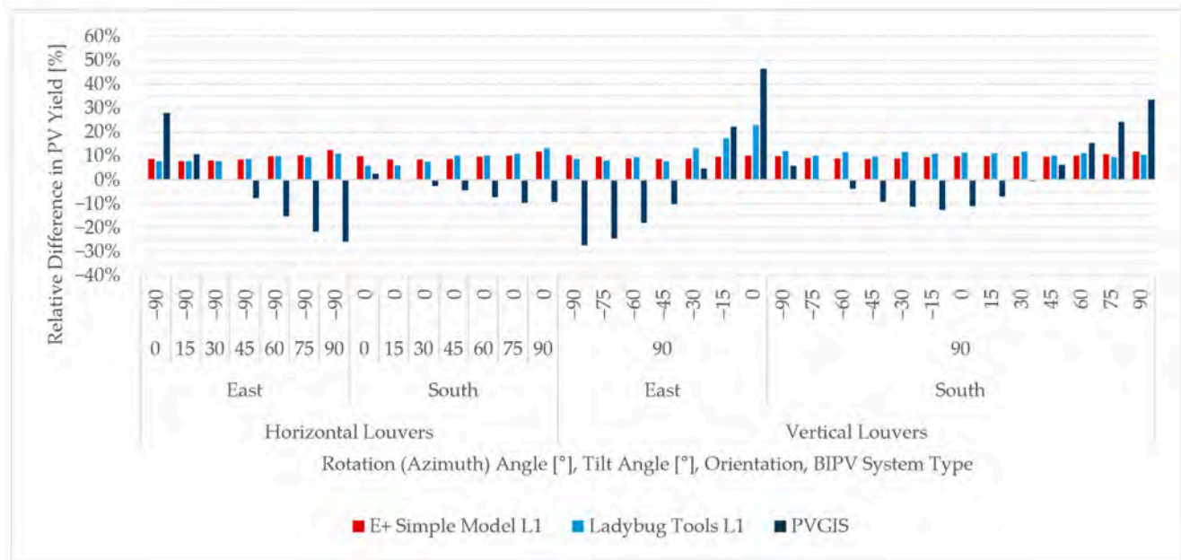
Figure 15. Relative differences in annual PV yield across assessment approaches for Level 1 PVSD configurations.
