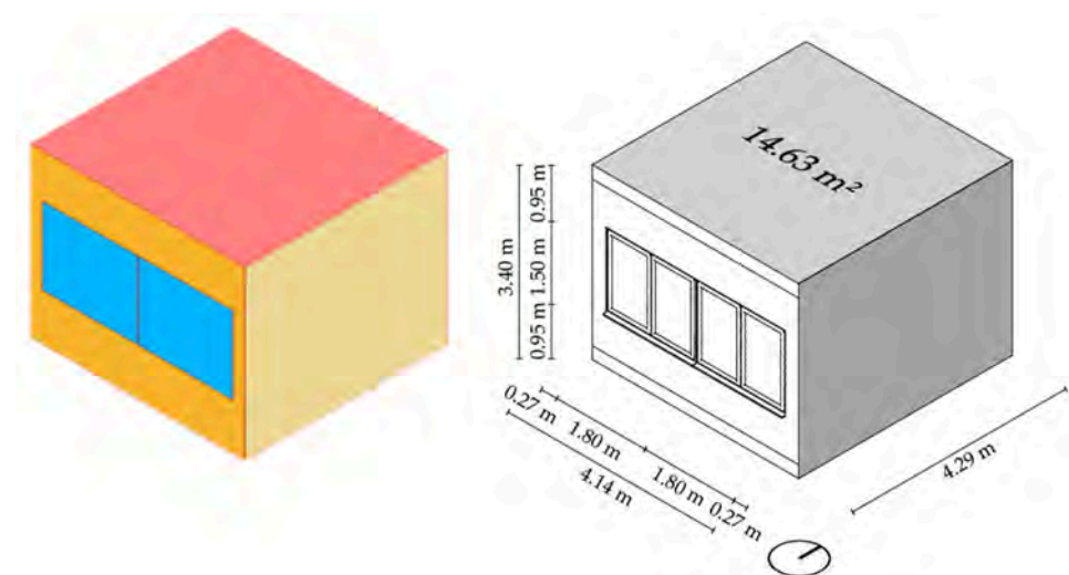
Figure 11. Room-scale simulation geometry used for the STPV modeling-choice analysis and cross-model comparison.
