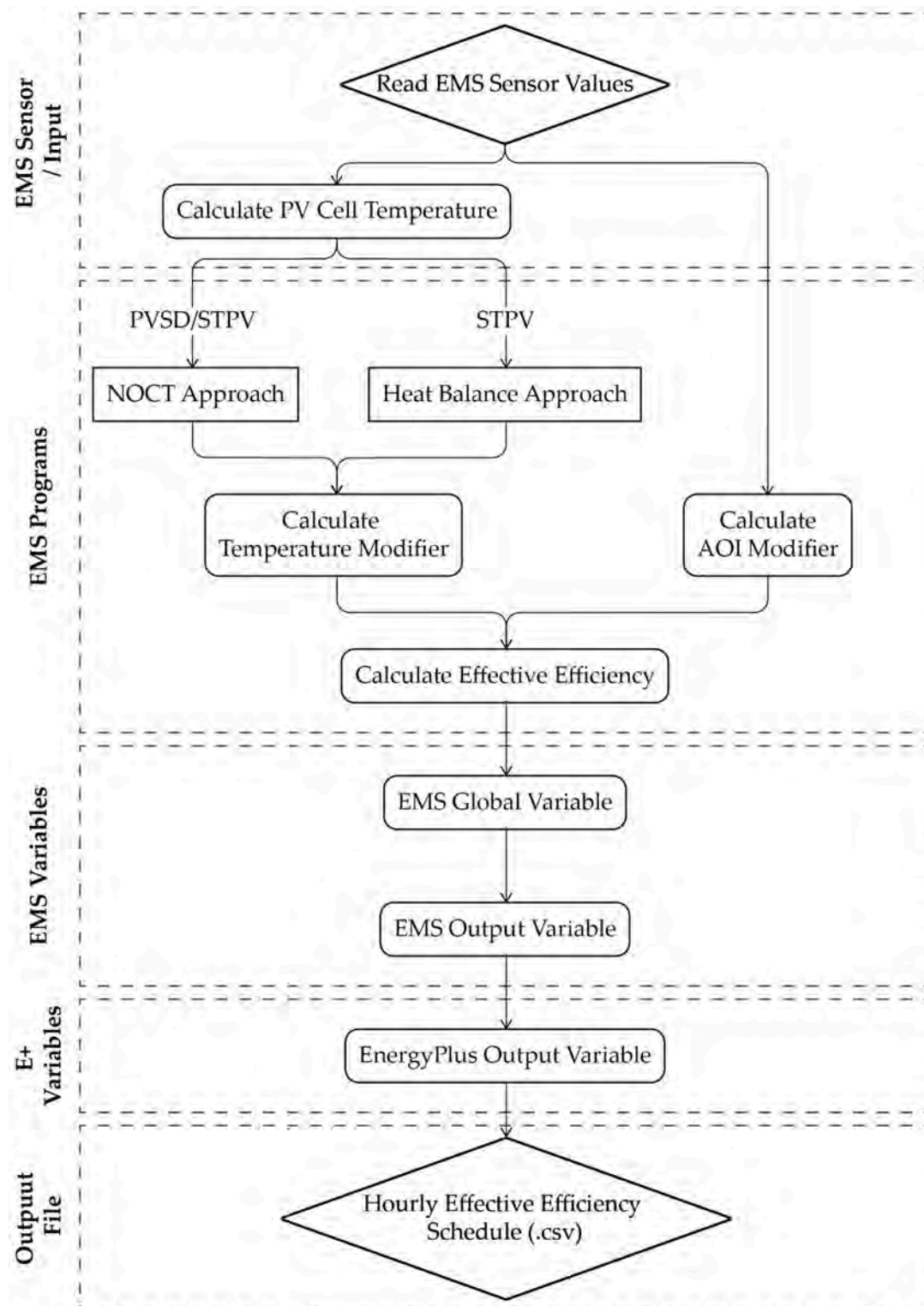
Figure 5. EnergyPlus EMS workflow for generating the hourly effective-efficiency schedule from AOI and temperature modifiers.
