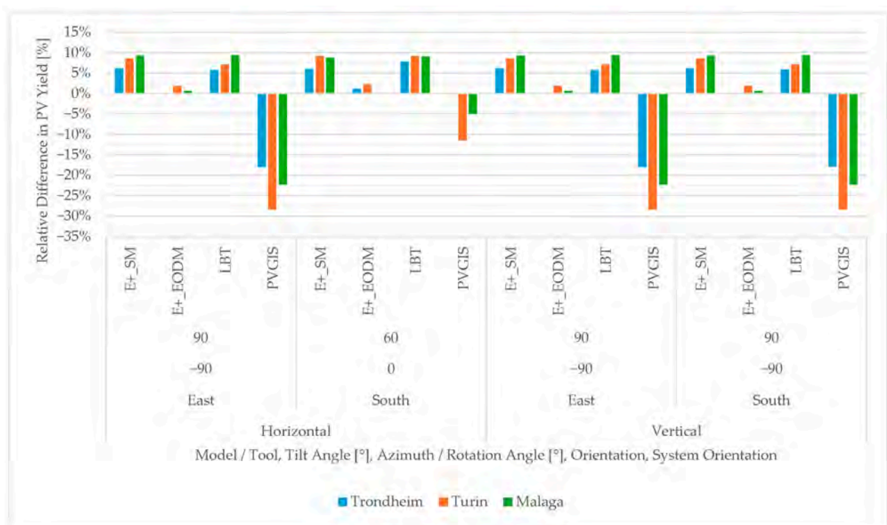
Figure 14. Relative differences in annual PV yield for selected Level 0 PVSD configurations across Turin, Trondheim, and Malaga.
