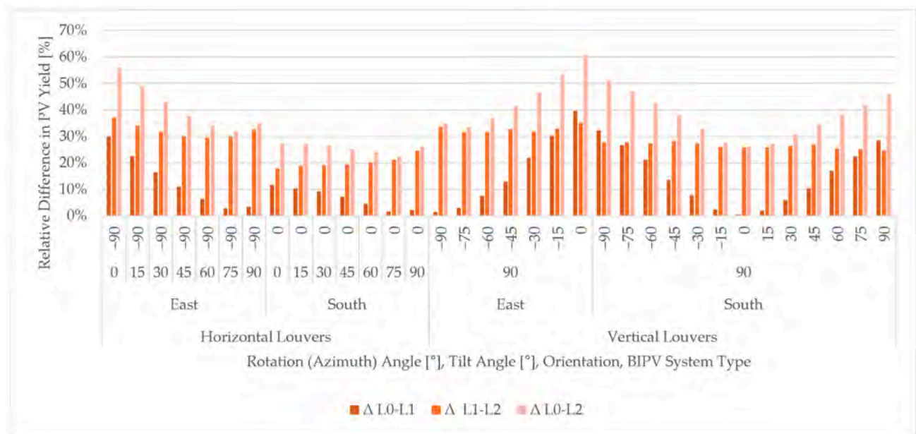
Figure 18. Relative PV yield reductions across PVSD geometry levels using the EnergyPlus modified simple model (MSM).
