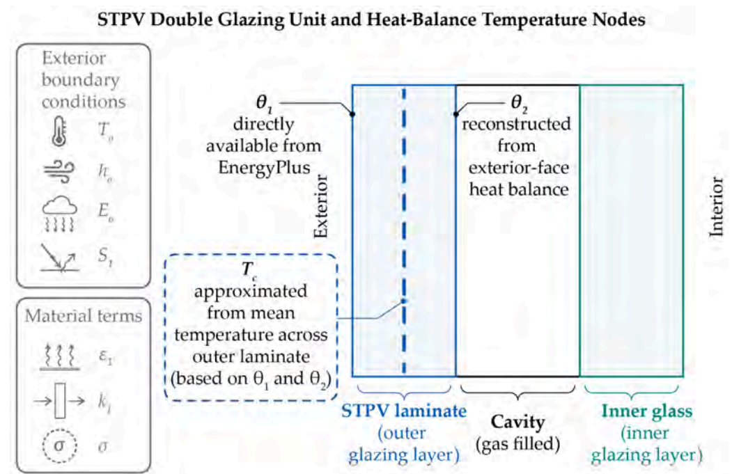
Figure 4. Heat-balance variables and temperature nodes used to reconstruct the inner-face temperature of the STPV outer glazing layer, redrawn by the authors based on the EnergyPlus engineering reference [31].
