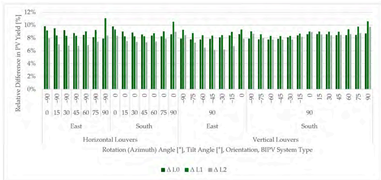
Figure 17. Relative differences in PV yield between EnergyPlus Simple model (SM) and the modified Simple model (MSM) across PVSD geometry levels.
