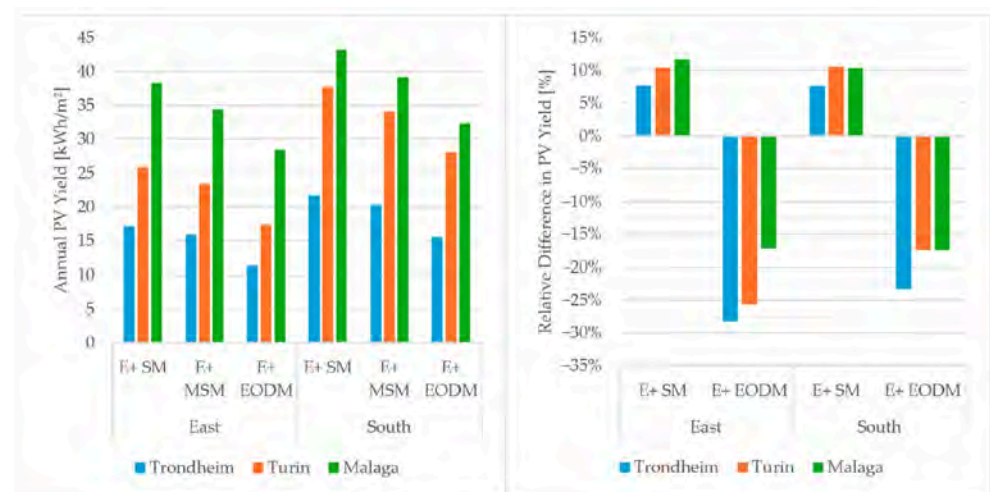
Figure 22. Relative differences in annual STPV yield across Turin, Trondheim, and Malaga.
