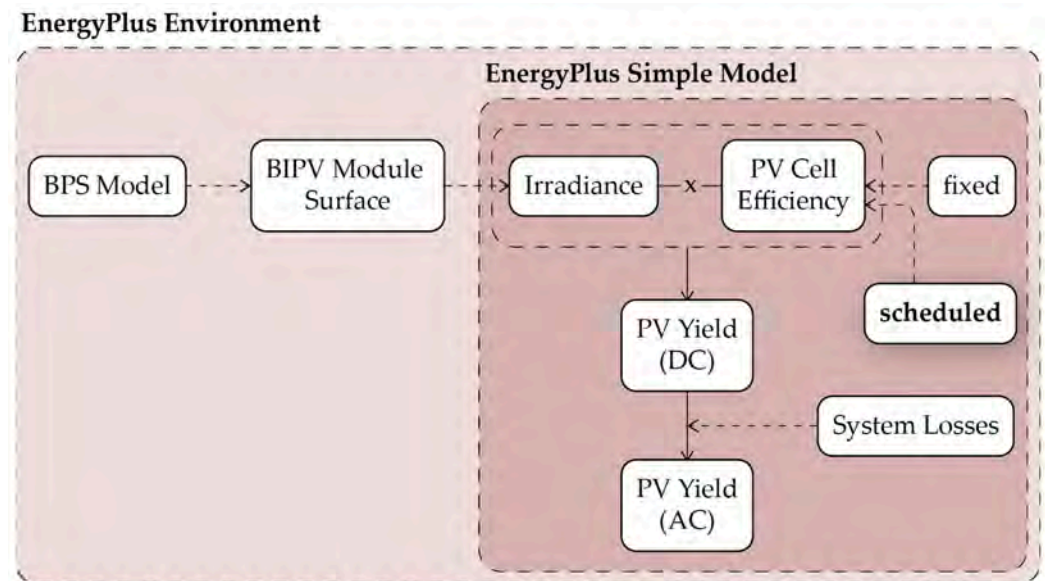
Figure 2. EnergyPlus Simple PV model structure and scheduled-efficiency input used as the basis for the modified Simple model.
