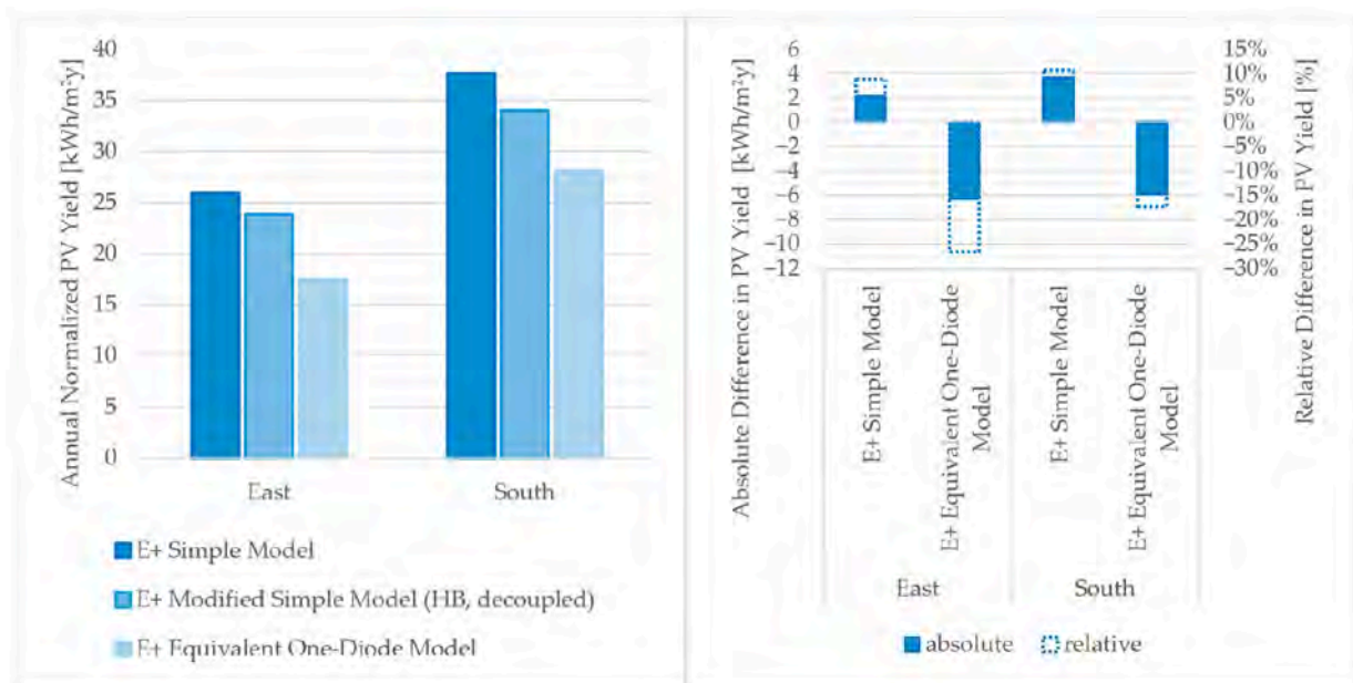
Figure 21. Cross-model comparison of STPV annual PV yield across EnergyPlus model configurations: (Left) annual normalized PV yield for SM, the selected MSM configuration, and EODM; (Right) absolute and relative differences with respect to the selected MSM configuration.
