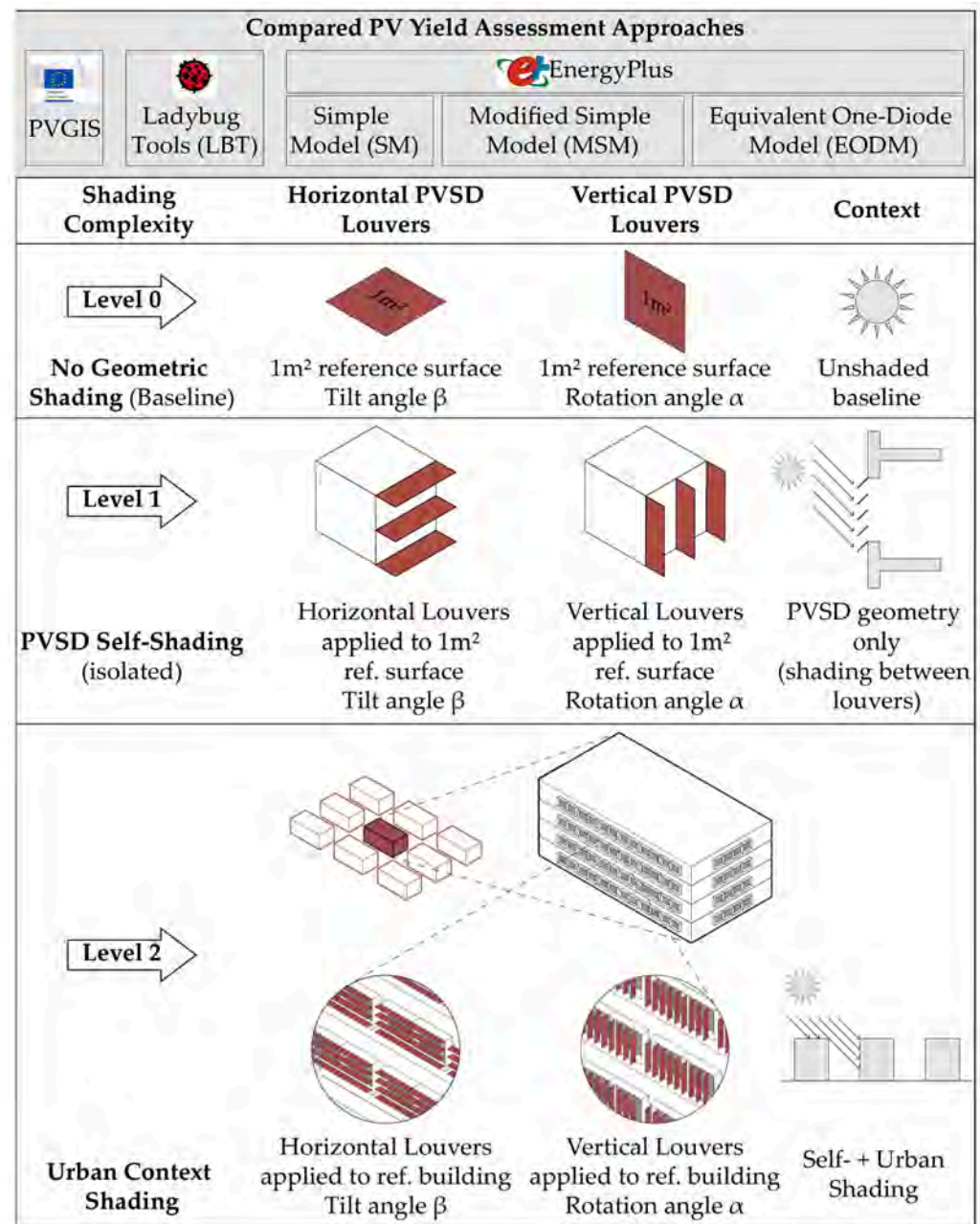
Figure 10. PVSD cross-tool comparison setup across geometry levels and assessment approaches.
