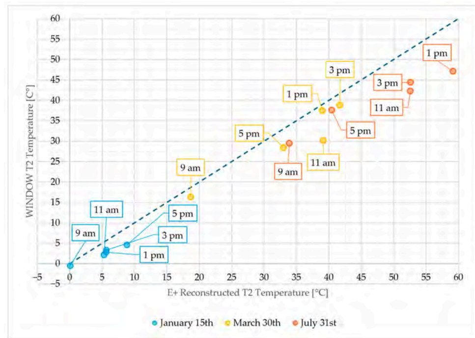
Figure A2. Comparison between EnergyPlus-reconstructed T2/\theta_2 and WINDOW T2/\theta_2 for selected boundary conditions. The dashed line indicates one-to-one agreement.
