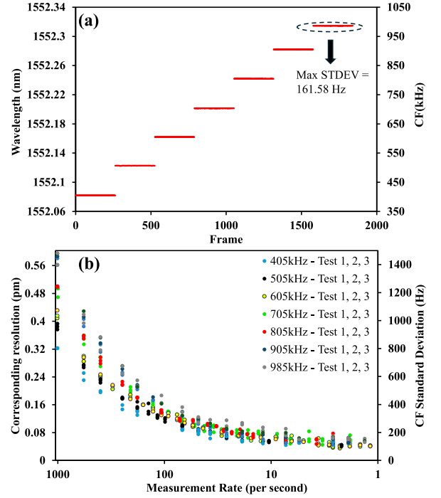
Fig. 8. Static FBG interrogation results (a) Estimated CF for different Bragg-wavelength settings, and (b) \sigma of the estimated CF across different Bragg wavelengths and measurement rates.
