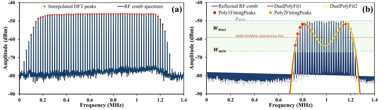
Fig. 6. RF comb spectra (a) generated by the DOFC and acquired with a record length of 16384 samples with a DFT averaging factor of 19 (red markers denote the detected comb line peaks), and (b) generated by the DOFC after reflection from the FBG, acquired with a record length of 4096 samples and a DFT averaging factor of 50. Fitting using the DualPoly4 curve applied.
