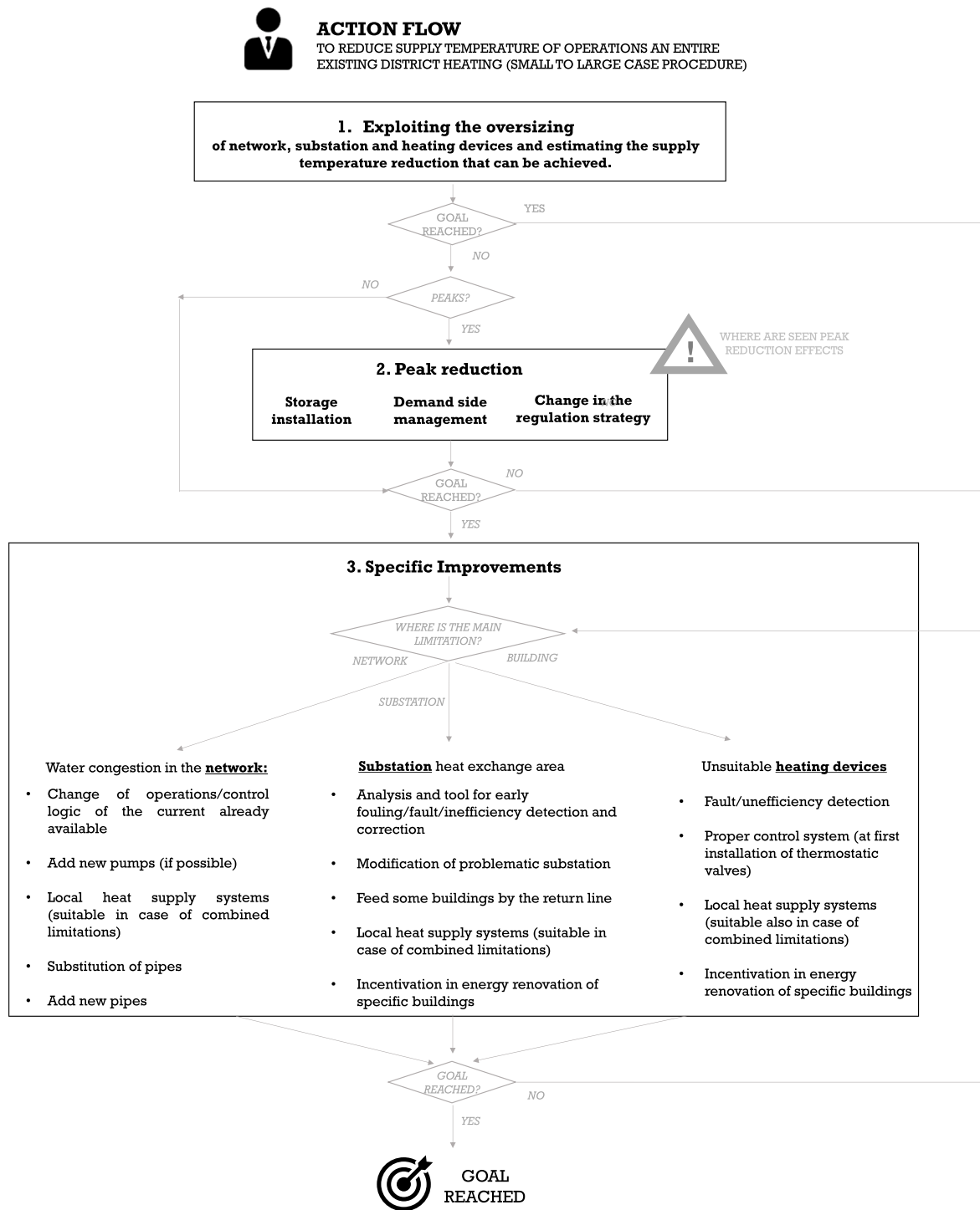
Fig. 10. Workflow for achieving supply temperature reduction in existing DH.
