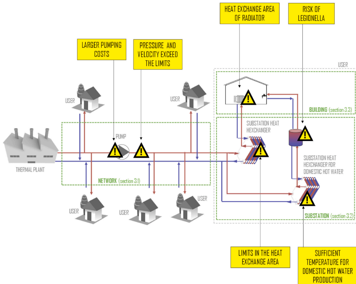
Fig. 2. Schematic of the limitations and issues encountered when reducing the supply temperature in existing DH.
