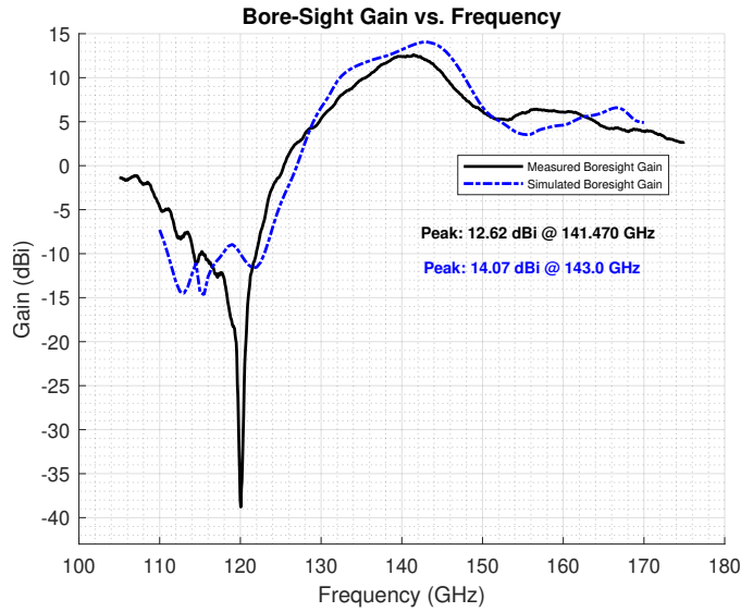
Fig. 5. FP antenna boresight gain.
