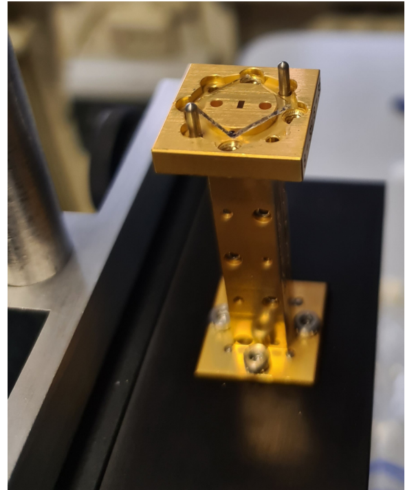
Fig. 1. Waveguide-based experimental setup in the 110-170 GHz frequency band.
