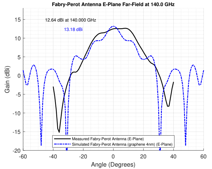
Fig. 8. Antenna E plane farfield at 140 GHz.
