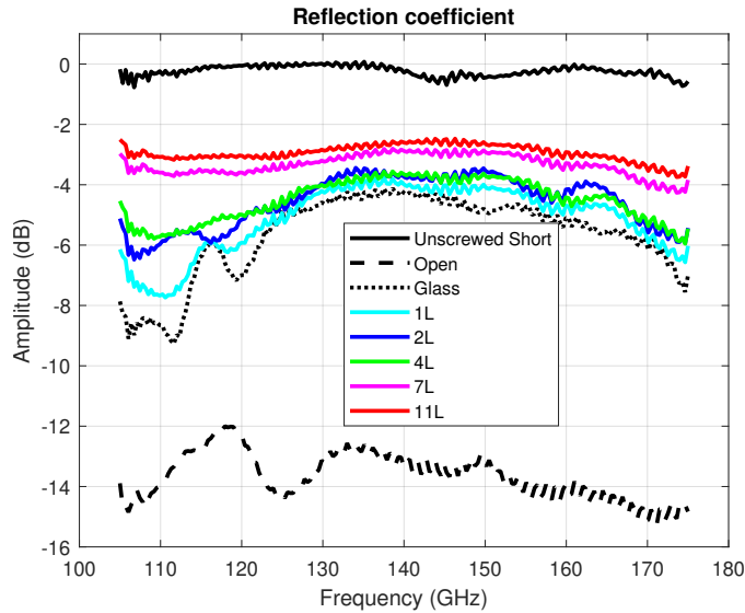
Fig. 2. Measured results of non-doped graphene samples in the 110-170 GHz frequency band.
