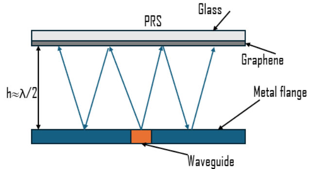
Fig. 4. Conceptual model of FP antenna.
