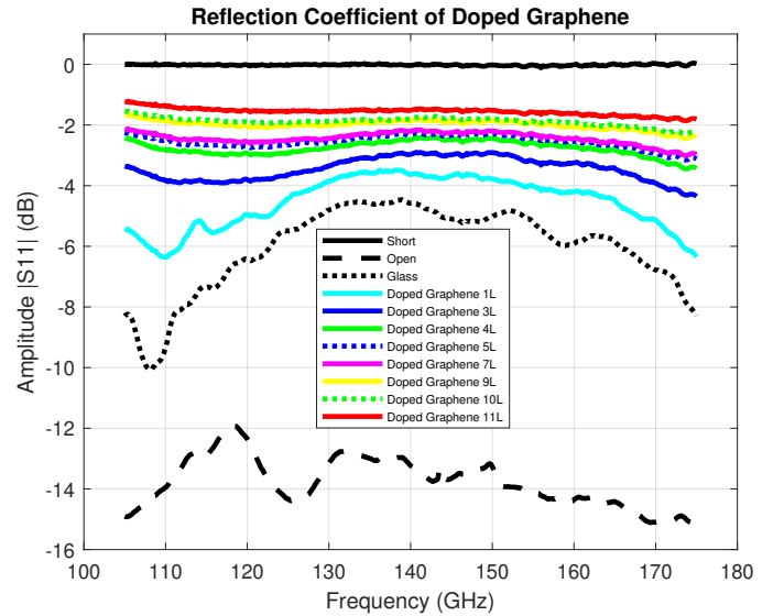
Fig. 3. Measured results of doped graphene samples in the 110-170 GHz frequency band.
