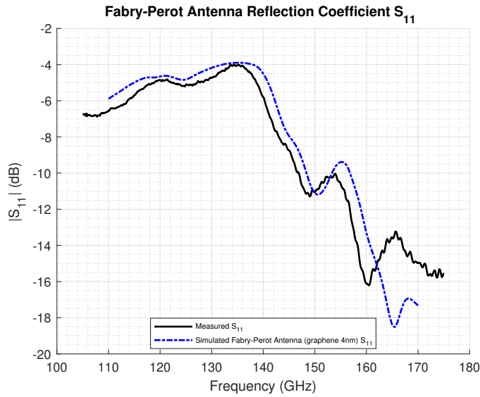
Fig. 6. FP antenna reflection coefficient.
