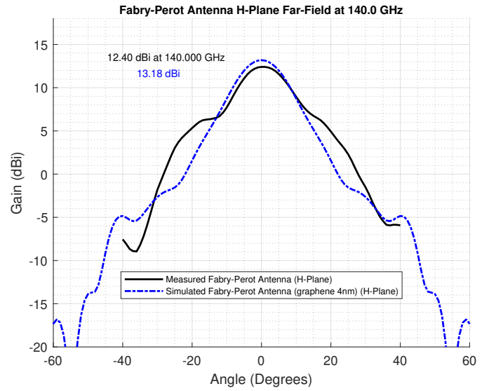
Fig. 7. Antenna H plane farfield at 140 GHz.
