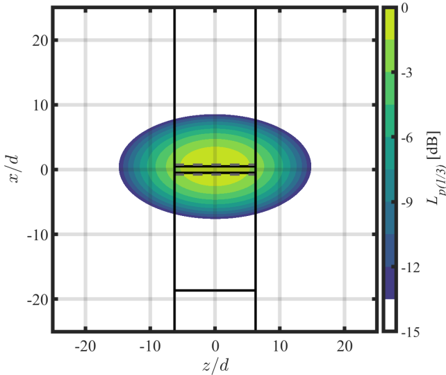
FIG. 5: Point-spread function at f_{1/3} = 1.6\text{kHz} for a simulated source emitting white noise at the origin of the coordinate system. The flow goes from the bottom to the top of the map.
