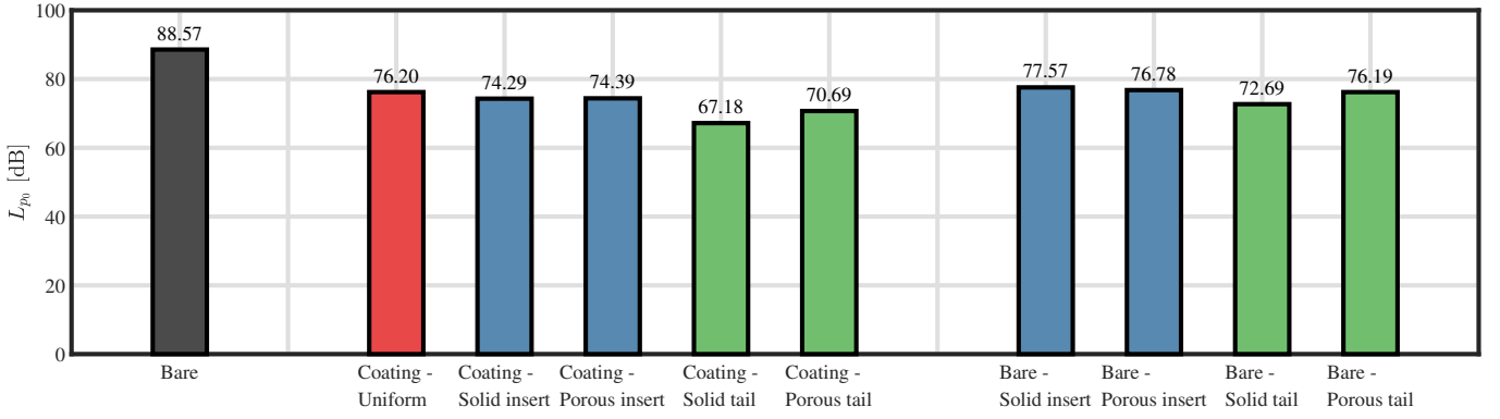
FIG. 9: Overall sound pressure level for the different cylinder configurations at Re_d = 4.1 \times 10^4 integrated between f = 131.25\text{Hz} and f = 20\text{kHz} . The L_{p0} values are indicated at the top of each bar. The notation for each cylinder configuration refers to Fig. 3a.
