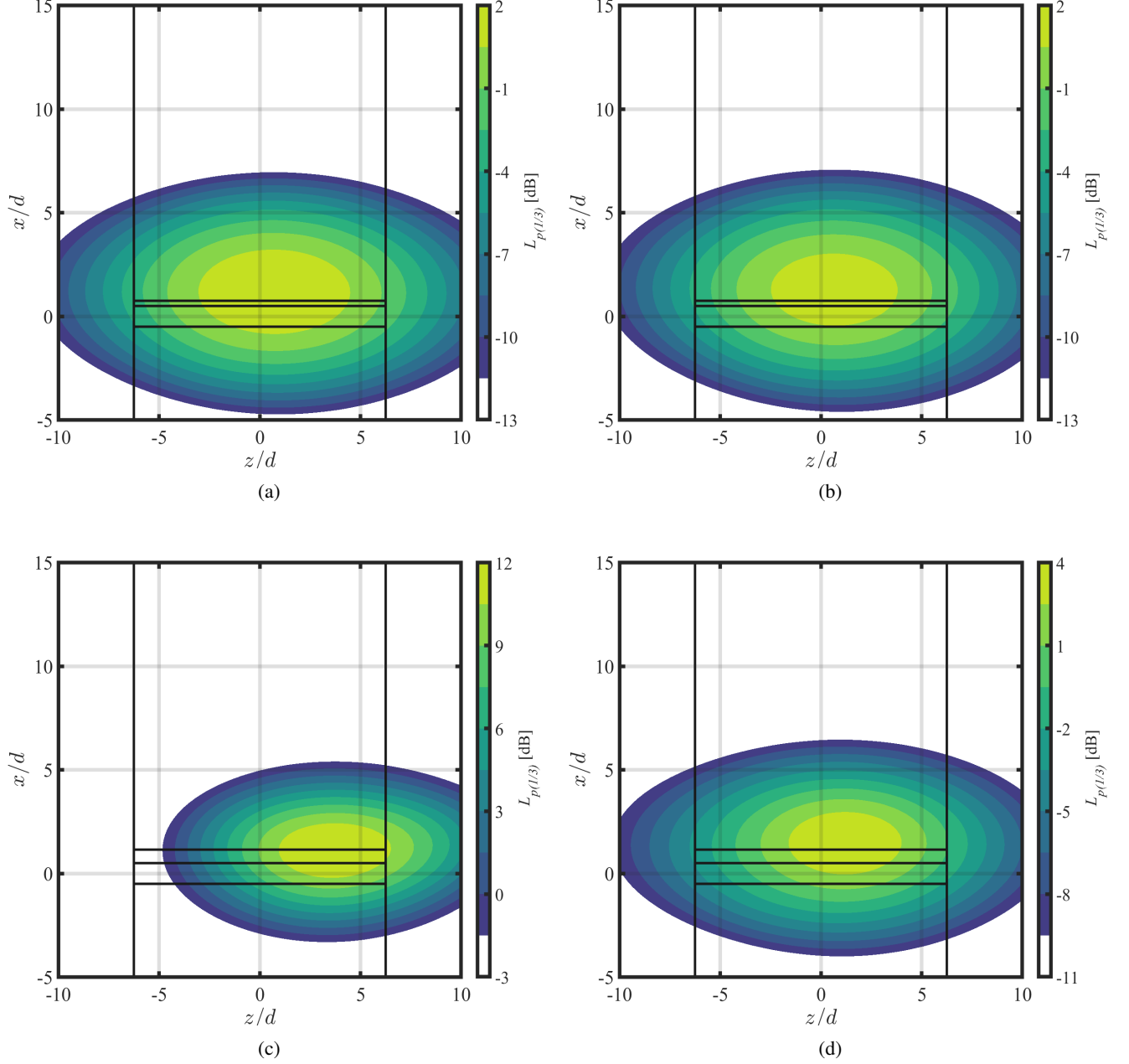
FIG. 16: GIB source-distribution maps for the bare cylinder integrated with the (a) solid insert, (b) porous insert, (c) solid tail, and (d) porous tail at f_{1/3} = 1.6 \text{ kHz} and Re_d = 6.8 \times 10^4 ( St = 0.64 ) computed with a reference pressure of p_{\text{ref}} = 20 \mu\text{Pa} .
