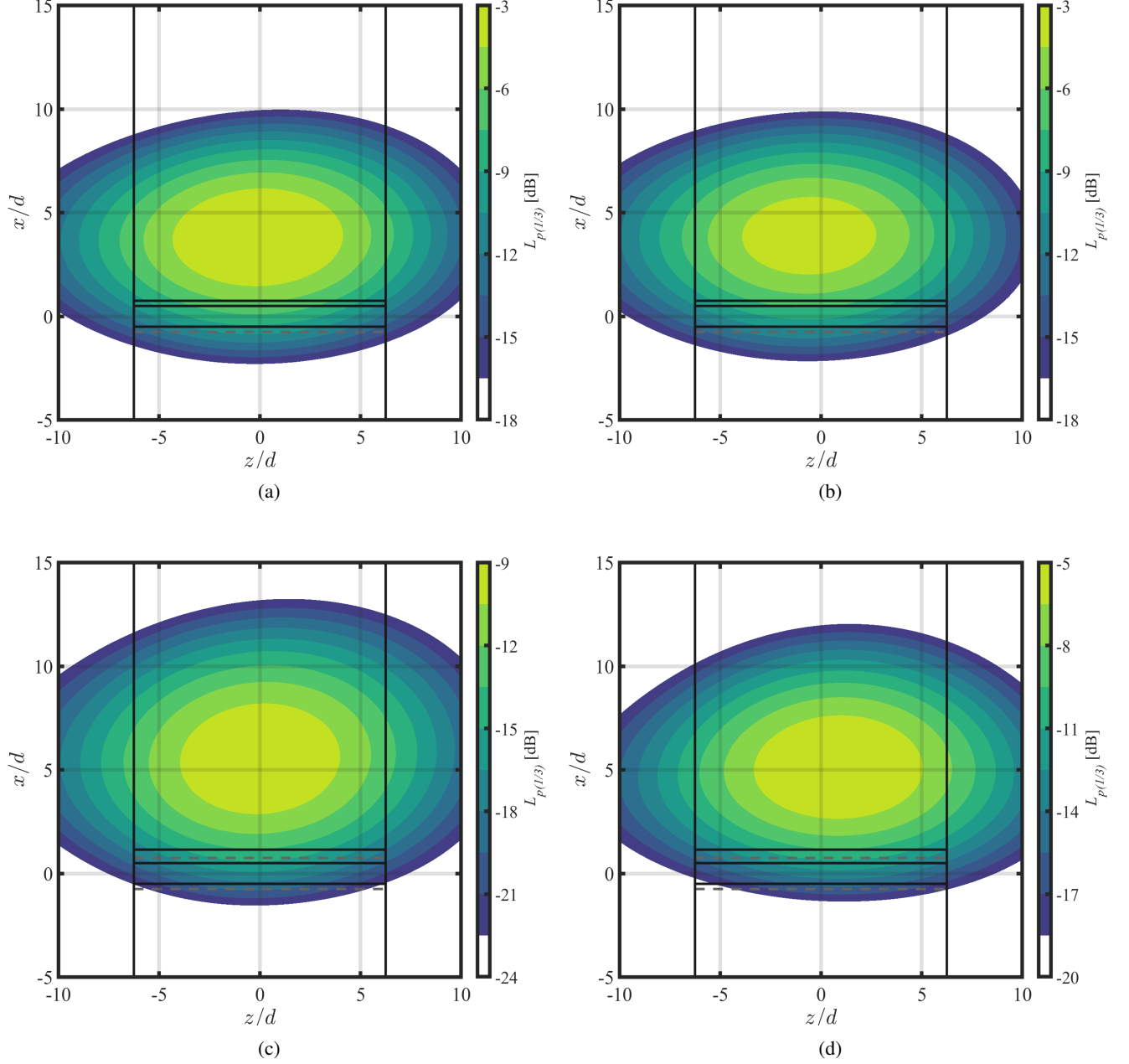
FIG. 15: GIB source-distribution maps for the cylinder coated with metal foam and integrated with the (a) solid insert, (b) porous insert, (c) solid tail, and (d) porous tail at f_{1/3} = 1.6 \text{ kHz} and Re_d = 6.8 \times 10^4 ( St = 0.64 ) computed with a reference pressure of p_{\text{ref}} = 20 \mu\text{Pa} .
