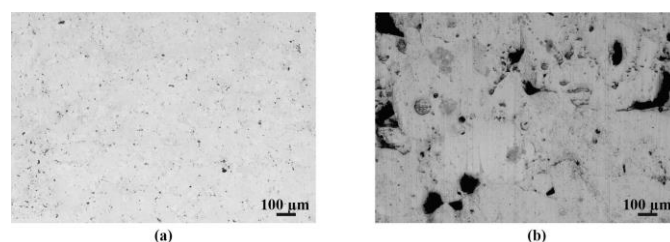
Fig. 4. (a) Pure Cu and (b) Cu-0.4% GNP samples.
