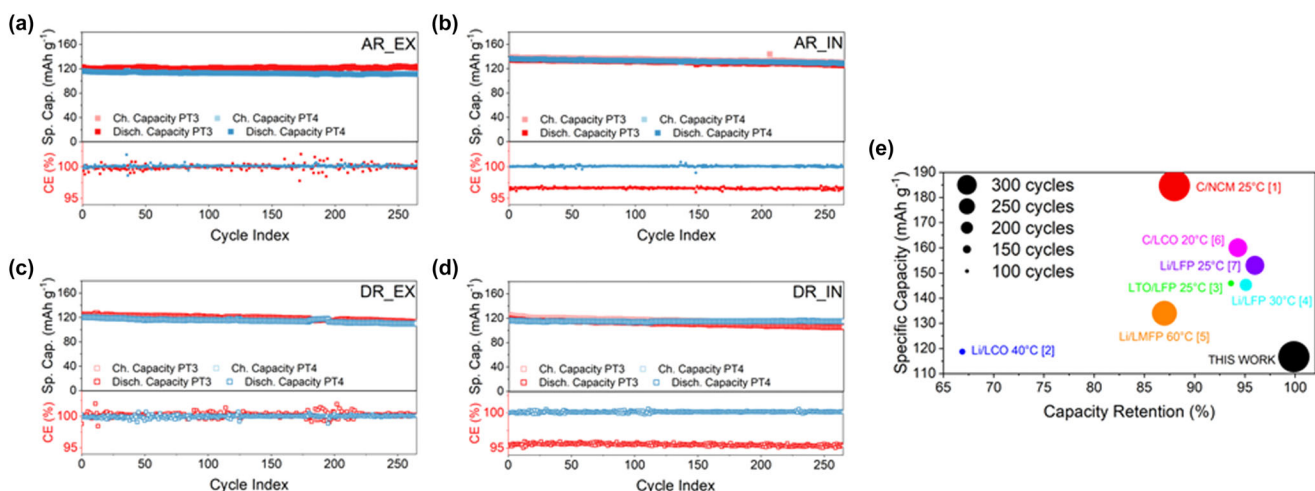
Figure 7. Long cycling capacity evolution and Coulombic efficiency for GPEs in a) AR_EX, b) AR_IN, c) DR_EX, and d) DR_IN configurations, e) Comparison between specific capacity, capacity retention after cycling and lifetime of PT4_DR_IN with in situ crosslinked GPEs.
