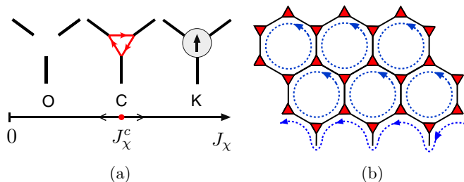
FIG. 1. Y junction and network. (a) Schematic illustration of the phase diagram. For J_\chi < J_\chi^c , the system flows to open boundary conditions (O fixed point), while for J_\chi > J_\chi^c , the three-channel Kondo (K) point is approached. The two stable fixed points are separated by an unstable chiral (C) fixed point at J_\chi = J_\chi^c . (b) A network of Y junctions with uniform J_\chi tuned to the C point realizes a chiral spin liquid.
