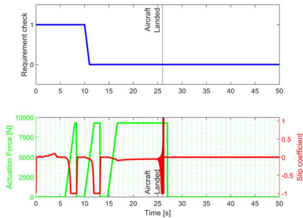
Fig. 13. Example of prediction of longitudinal wheel slip coefficient and brake actuation force during landing, to verify the LG-5.1.1 requirement.
