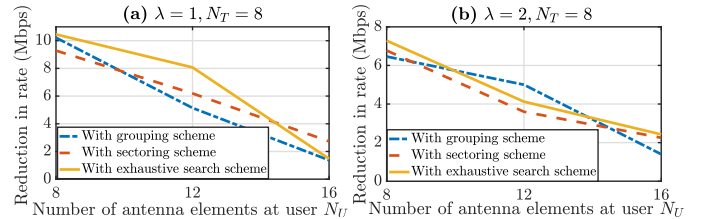
Figure 4: Reduction in rate when using estimated AoAs as compared to using true AoAs to design tags' reflection coefficients and user steering direction in case of homogeneously distributed tags.
